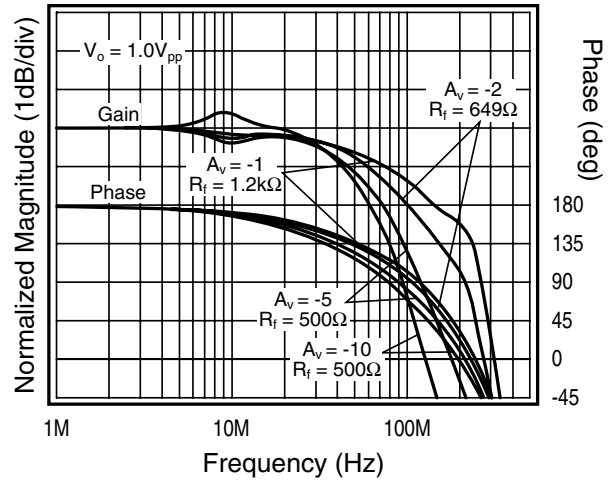
Inverting Frequency Response
