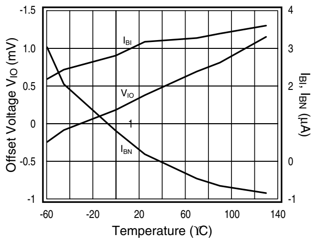
I_{BI} , I_{BN} , V_{IO} vs. Temperature
