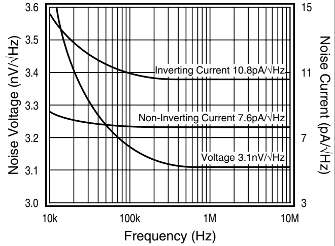
Equivalent Input Noise
