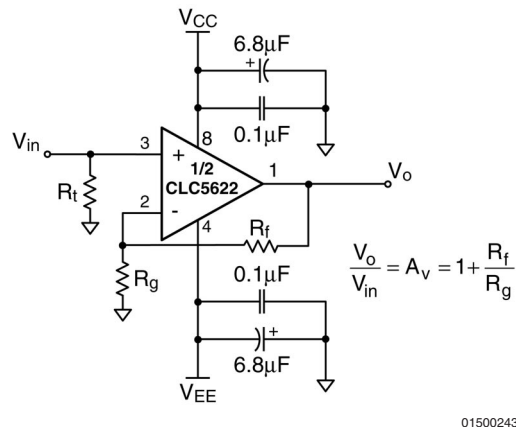
FIGURE 5. Dual Supply Non-Inverting Configuration
