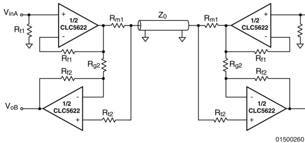
FIGURE 16. Full Duplex Cable Driver
