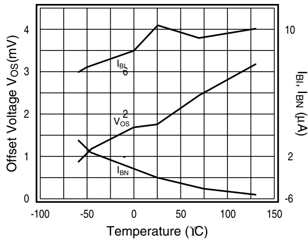
I_B , I_{BN} , V_{OS} vs. Temperature
