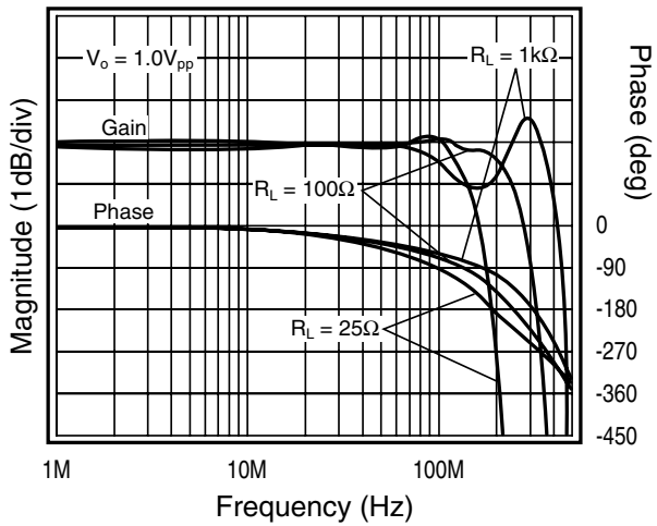
Frequency Response vs. R_L
