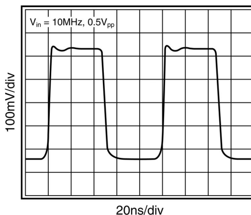
FIGURE 11. Response After 10m of Cable
