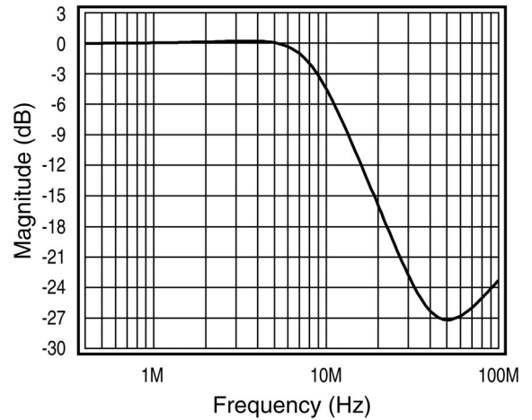
FIGURE 14. Lowpass Response
