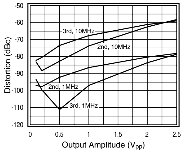
2nd & 3rd Harmonic Distortion, R_L = 1k\Omega
