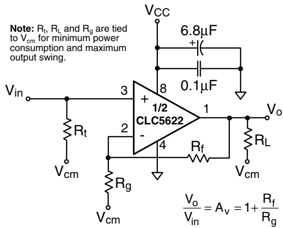
FIGURE 1. Non-Inverting Configuration
