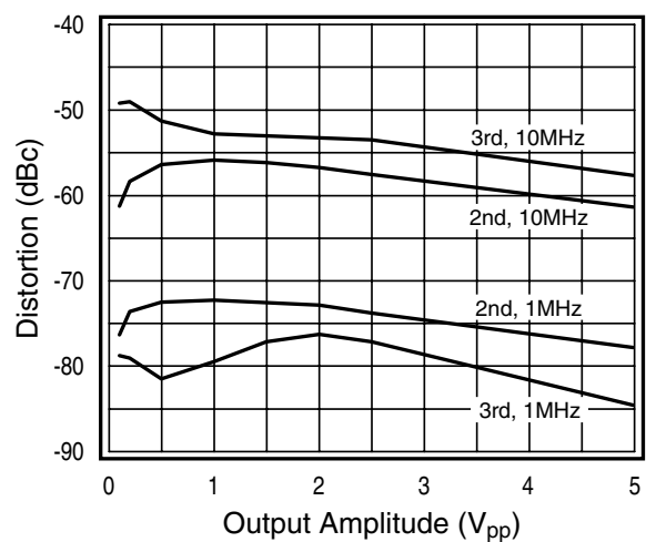
2nd & 3rd Harmonic Distortion, R_L = 25\Omega
