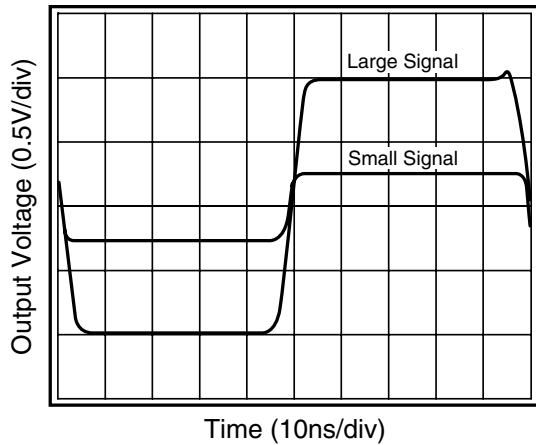
Large & Small Signal Pulse Response
