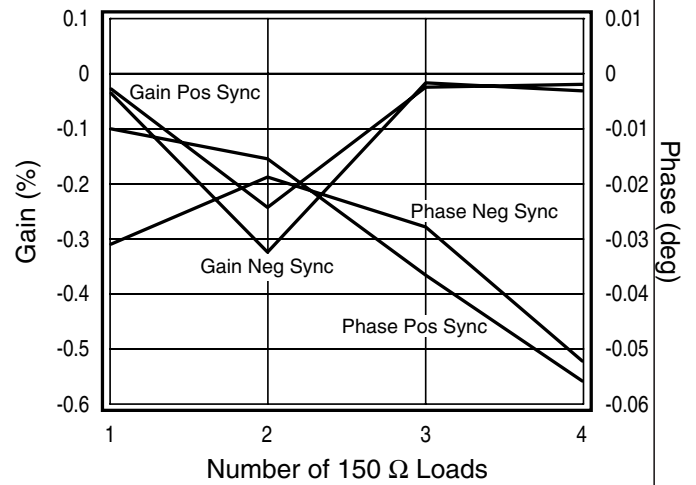
Differential Gain and Phase
