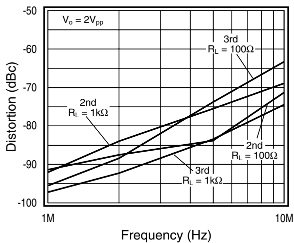
2nd &amp; 3rd Harmonic Distortion
