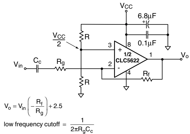
FIGURE 4. Dual Supply Non-Inverting Configuration
