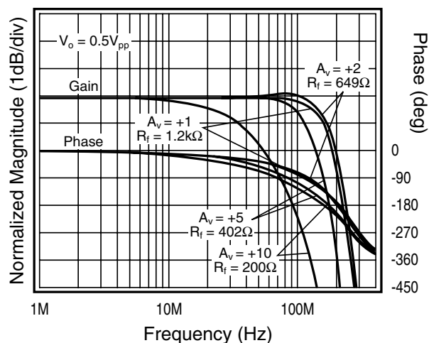
Non-Inverting Frequency Response
