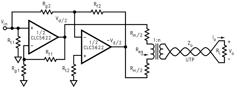
Differential Line Driver with Load Impedance Conversion
