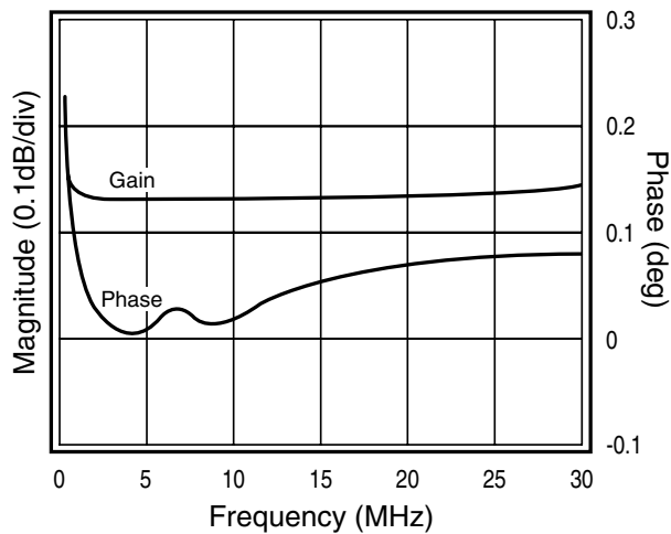
Gain Flatness &amp; Linear Phase
