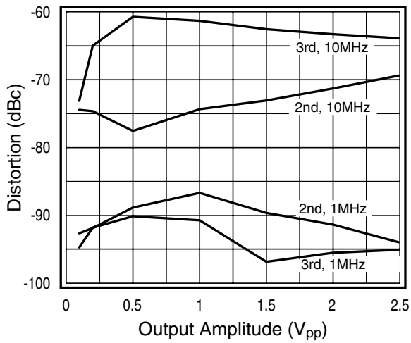
2nd & 3rd Harmonic Distortion, R_L = 100\Omega
