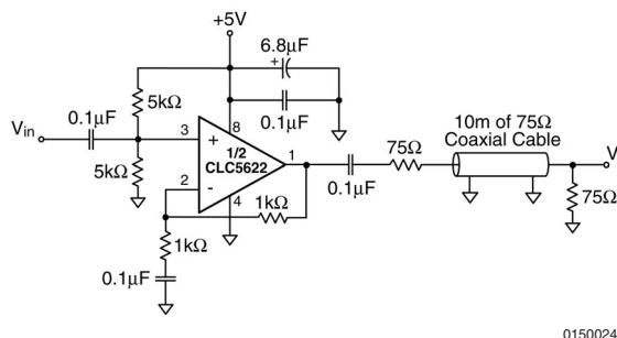
FIGURE 10. Single Supply Cable Driver
