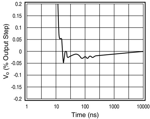
Short Term Settling Time
