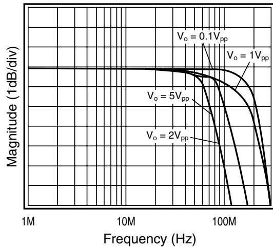
Frequency Response vs. V_o
