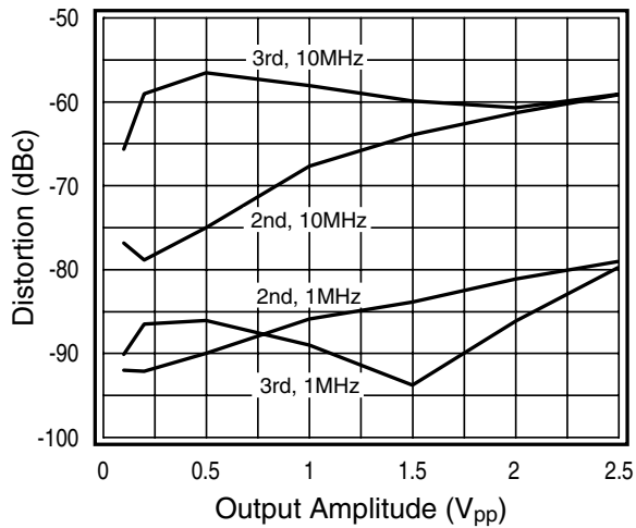
2nd & 3rd Harmonic Distortion, R_L = 100\Omega
