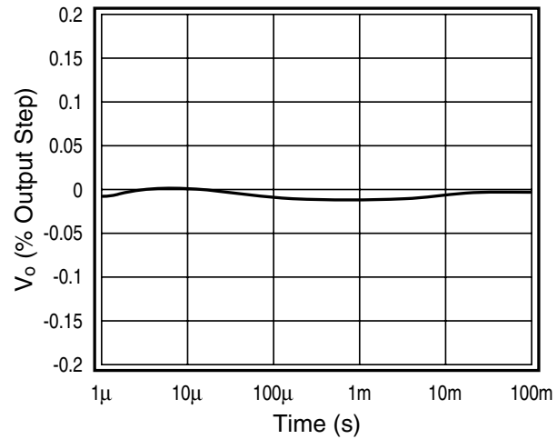
Long Term Settling Time
