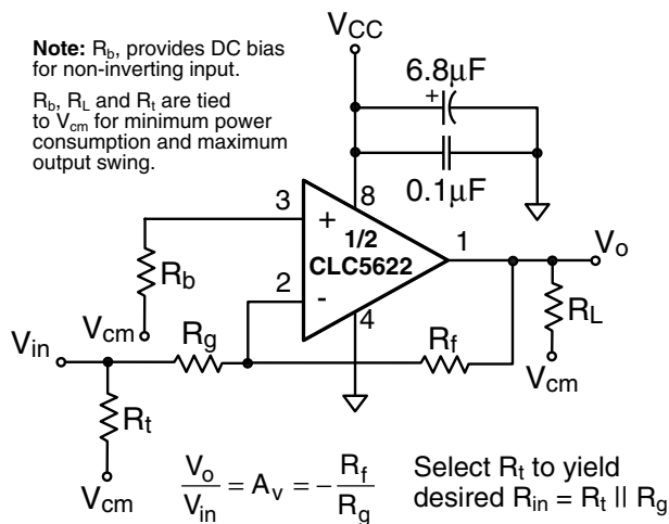
FIGURE 2. Inverting Configuration
