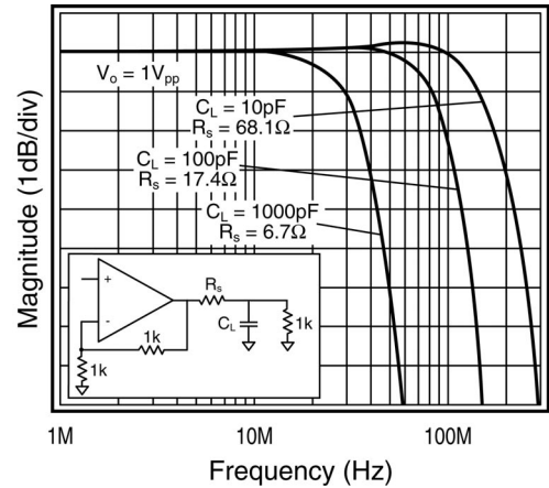
FIGURE 7. Frequency Response vs. C_L
