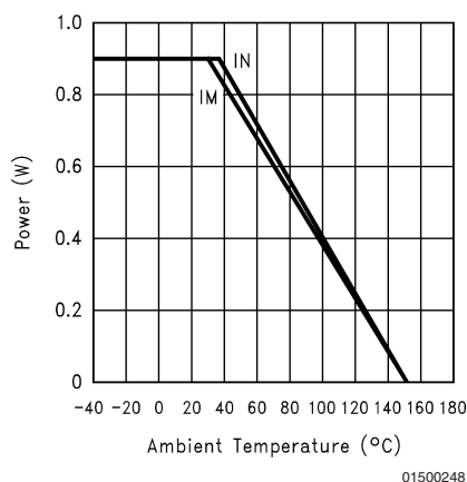
FIGURE 9. Power Derating Curves
