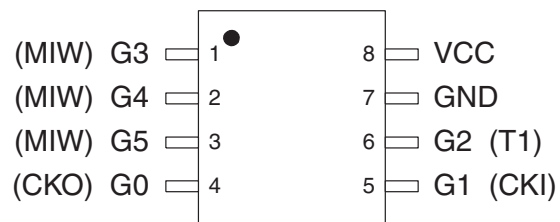
Figure 2: ACE1001 SOIC 8-Pin Device Pinout (a) Normal Operation
