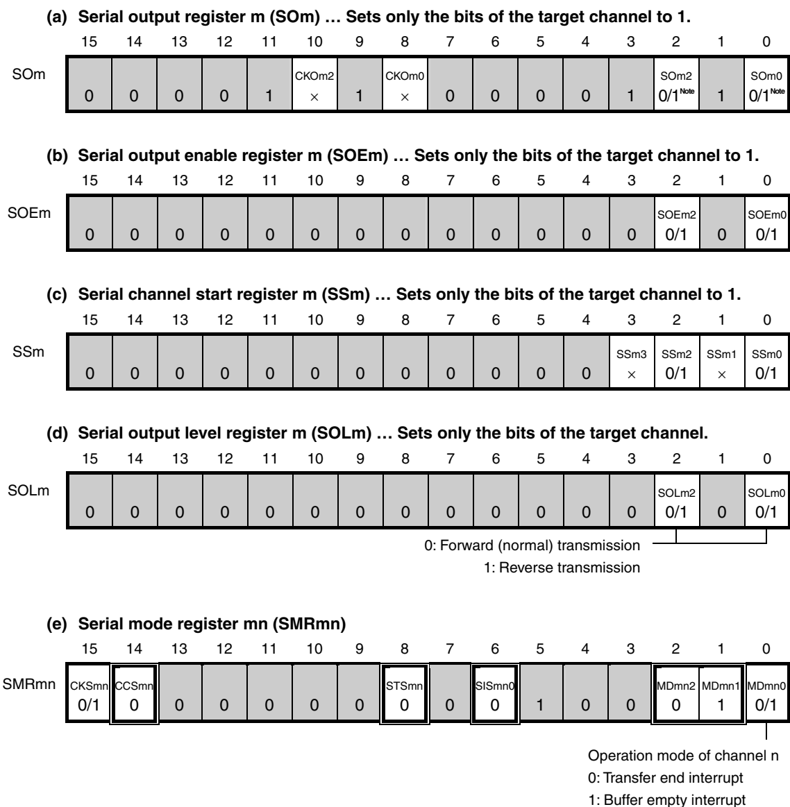
Figure 14-68. Example of Contents of Registers for UART Transmission of UART (UART0, UART1, UART2, UART3) (1/2)
