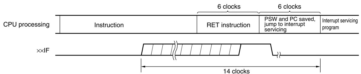
Figure 18-9. Interrupt Request Acknowledgment Timing (Maximum Time)
