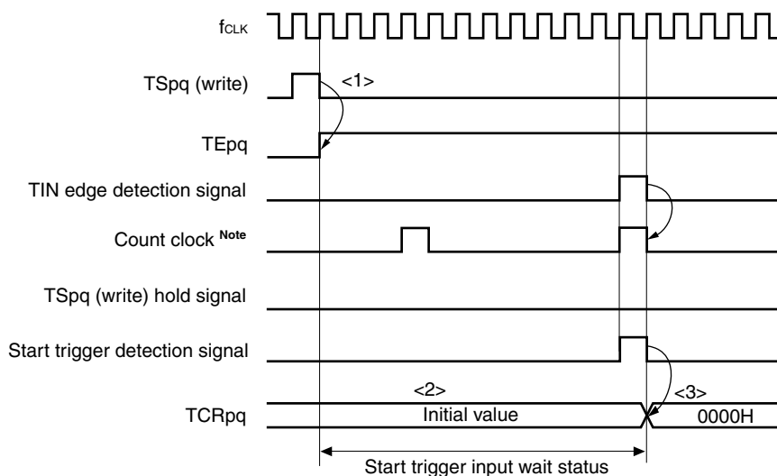
Figure 6-15. Start Timing (In Capture &amp; One-count Mode)
