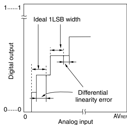
Figure 10-25. Differential Linearity Error
