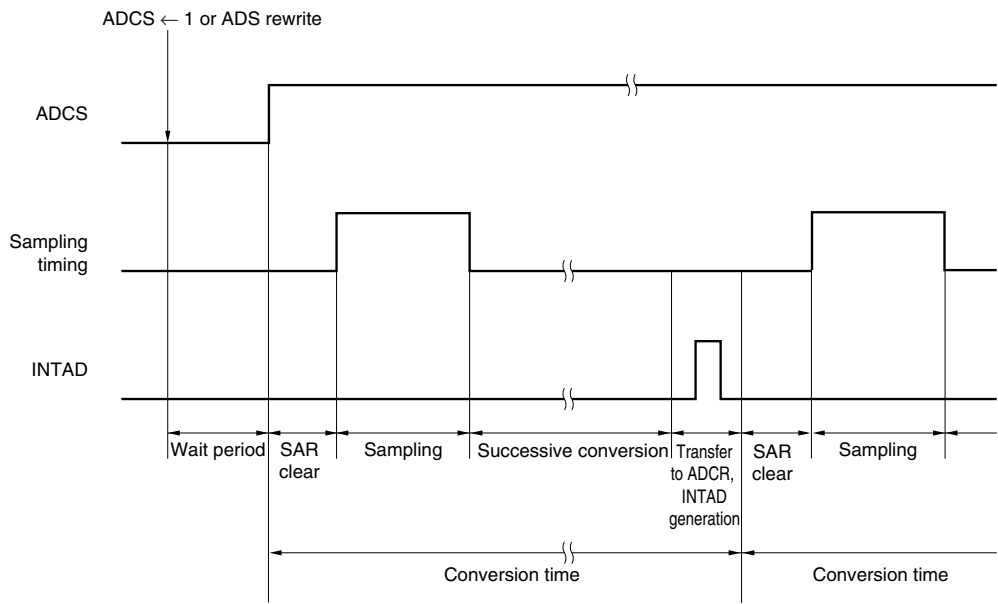
Figure 10-6. A/D Converter Sampling and A/D Conversion Timing
