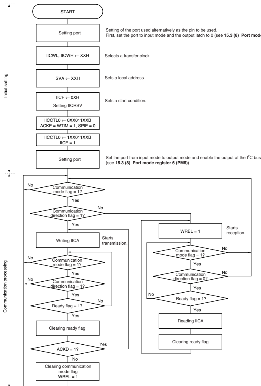
Figure 15-30. Slave Operation Flowchart (1)
