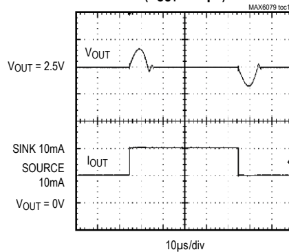
MAX6079_25 ±10mA LOAD TRANSIENT (C OUT = 0.1μF)
