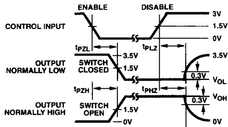
FIGURE 2. ENABLE AND DISABLE TIMING
