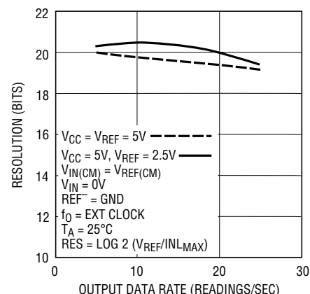
Figure 38. Resolution ( \text{INL}_{MAX} \leq 1\text{LSB} ) vs Output Data Rate and Reference Voltage
