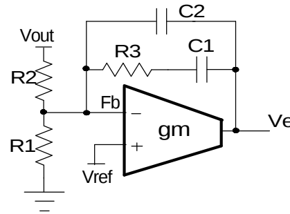
Figure 7 - Type II compensator with transconductance amplifier(case 1)
