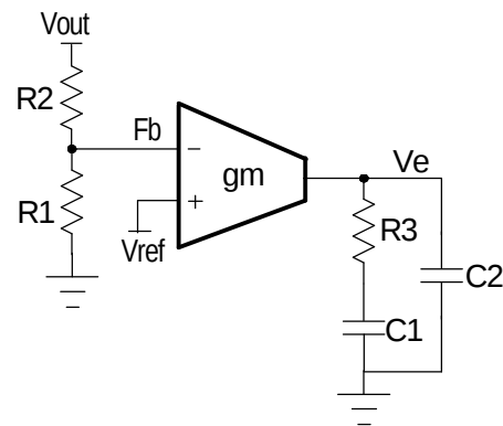
Figure 9 - Type II compensator with transconductance amplifier
