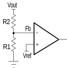
Figure 10 - Voltage divider
