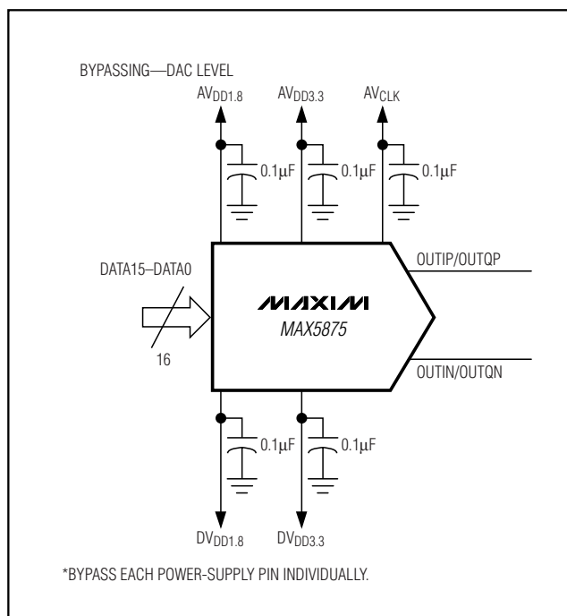
Figure 8. Recommended Power-Supply Decoupling and Bypassing Circuitry
