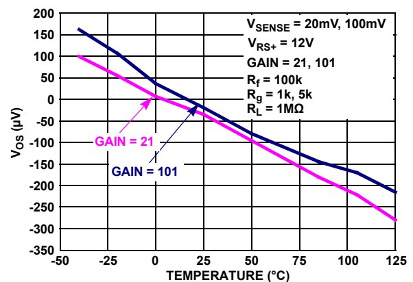
Figure 66. V_{OS} ( \mu V ) vs Temperature
