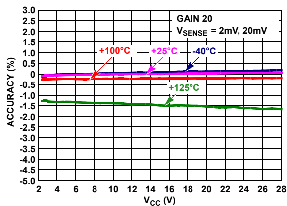
Figure 46. Gain Accuracy vs V_{CC} , High-Side
