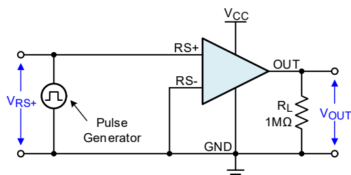
Figure 75. Slew Rate
