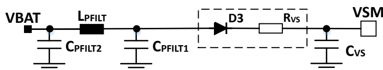
Figure 5 Reverse polarity for 48 V applications
