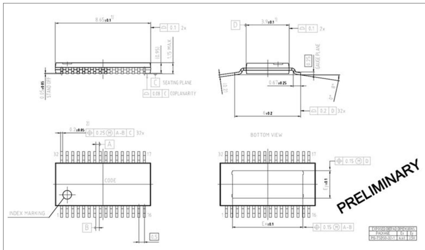
Figure 27 TSDSO-32
