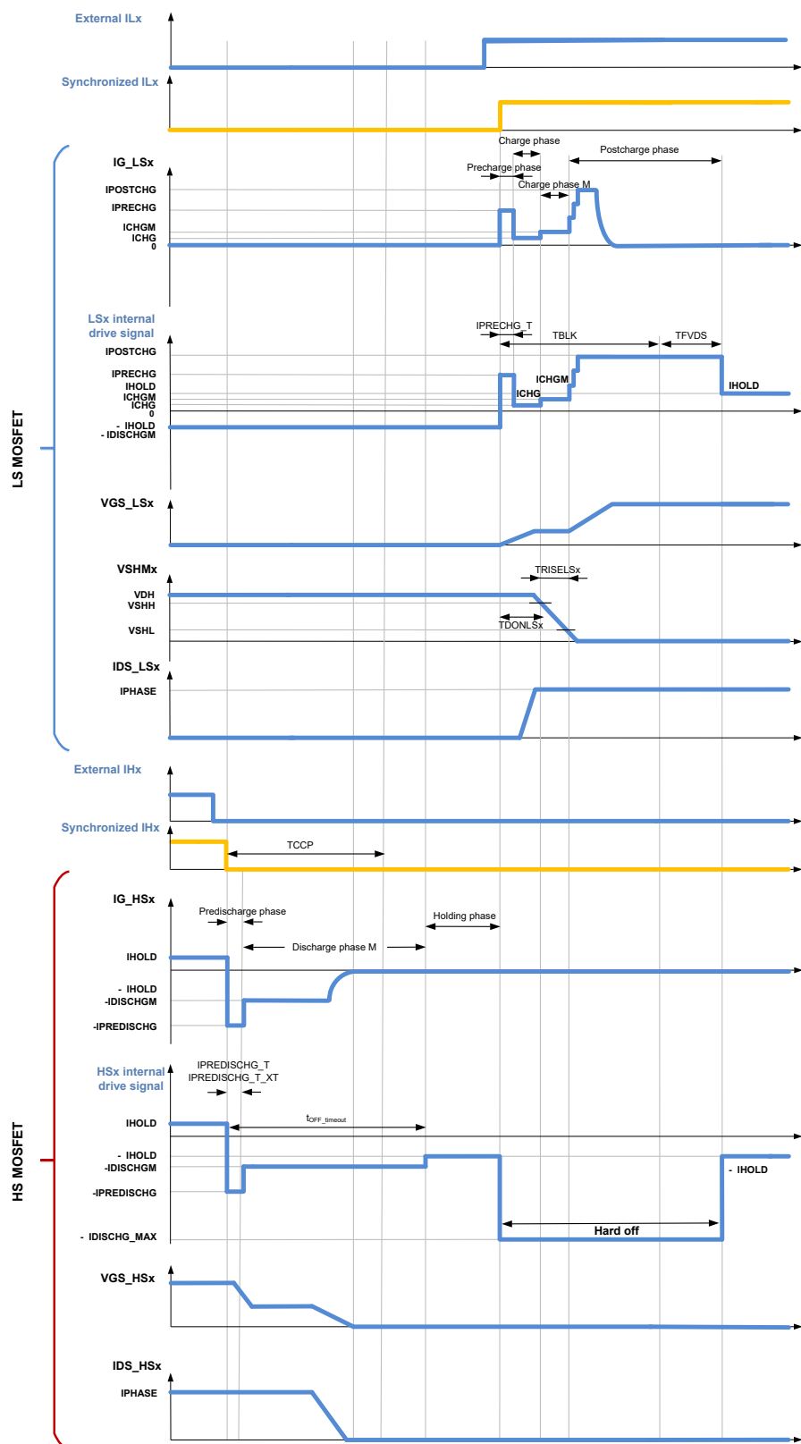
Figure 14 Turn-on of the low-side MOSFET
