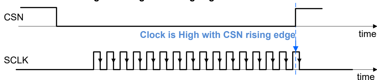
Figure 22 Polarity error
