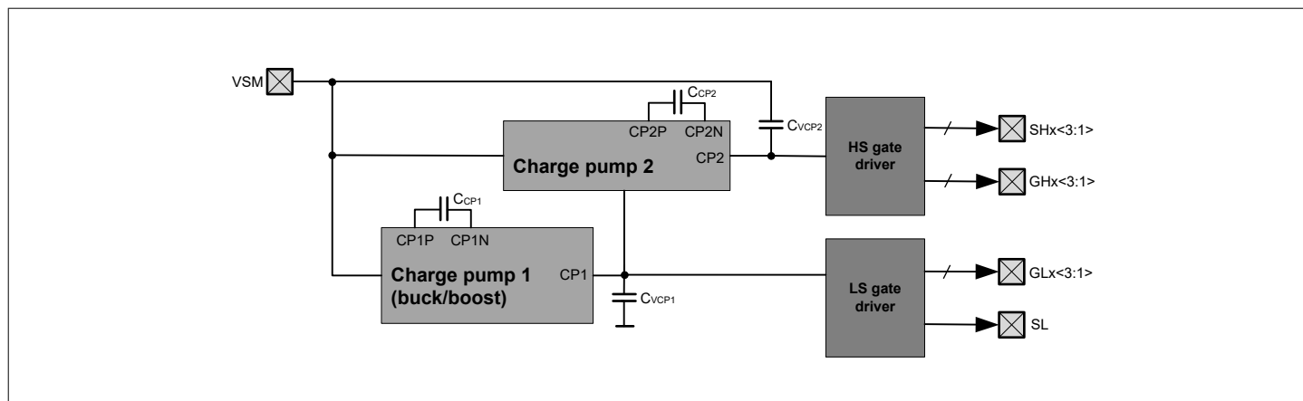
Figure 4 Power supply
