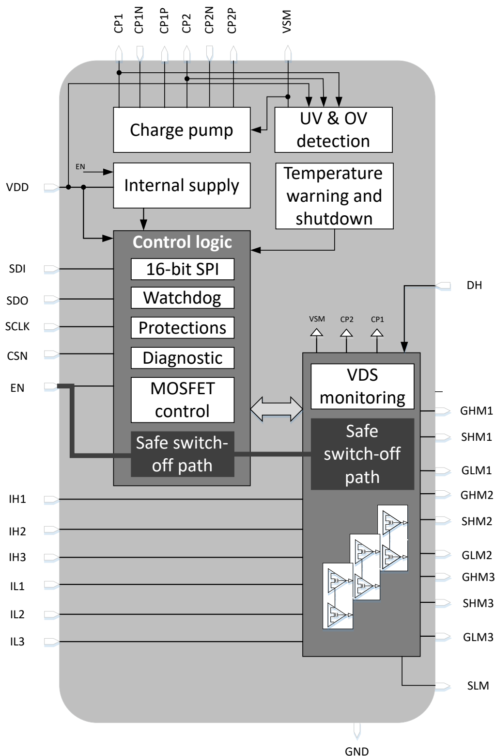
Figure 1 Block diagram
