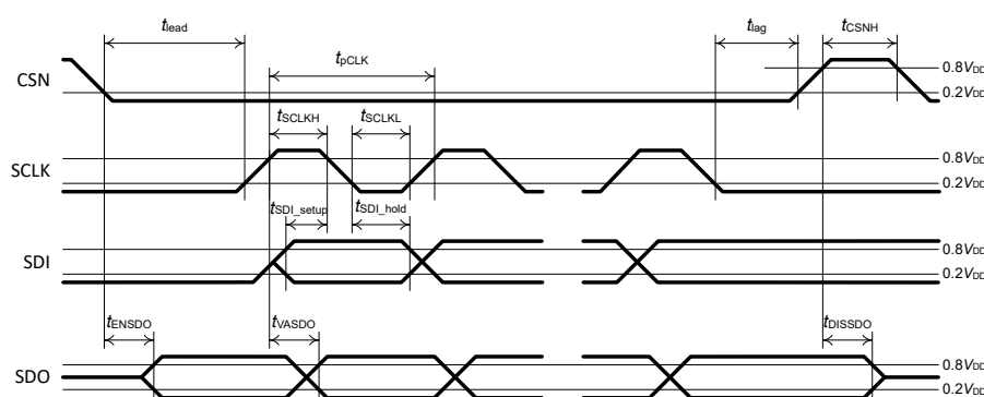
Figure 20 SPI timing parameters
