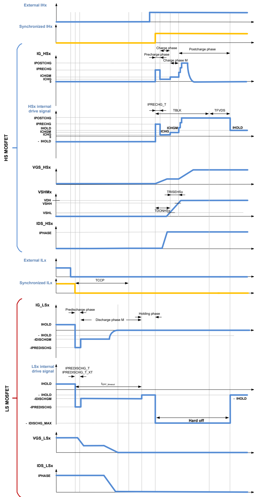
Figure 12 Turn-on of the high-side MOSFET
