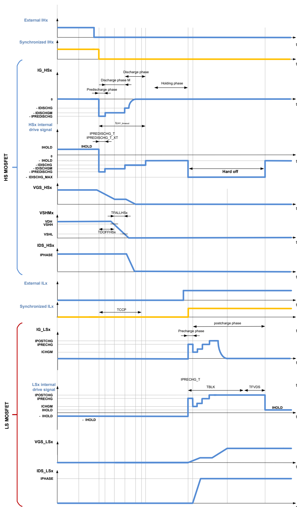
Figure 13 Turn-off of the high-side MOSFET
