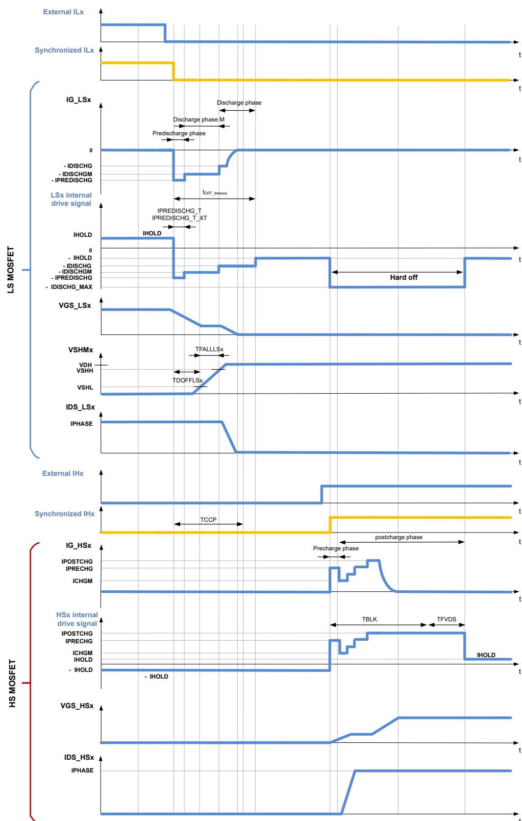
Figure 15 Turn-off of the low-side MOSFET
