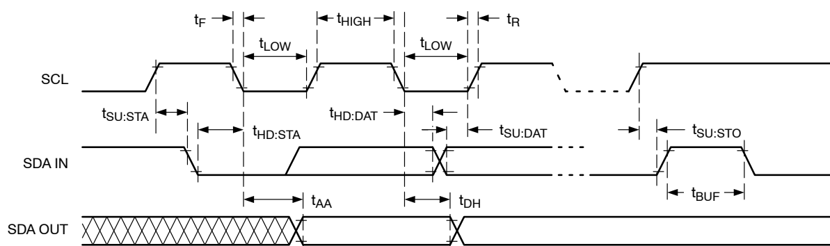
Figure 2. Bus Timing
