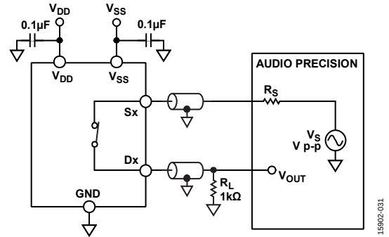
Figure 33. THD + Noise
