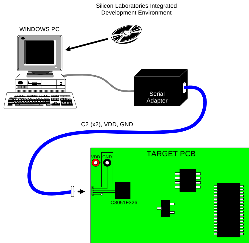
Figure 1.9. Development/In-System Debug Diagram
