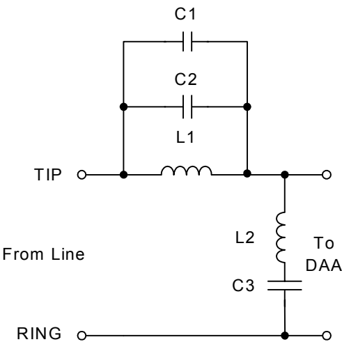
Figure 23. Billing Tone Filter
