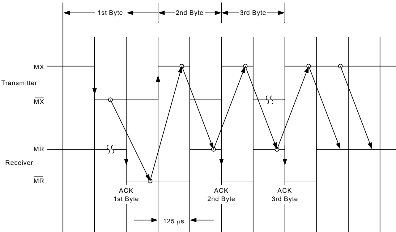
Figure 42. Monitor Handshake Timing
