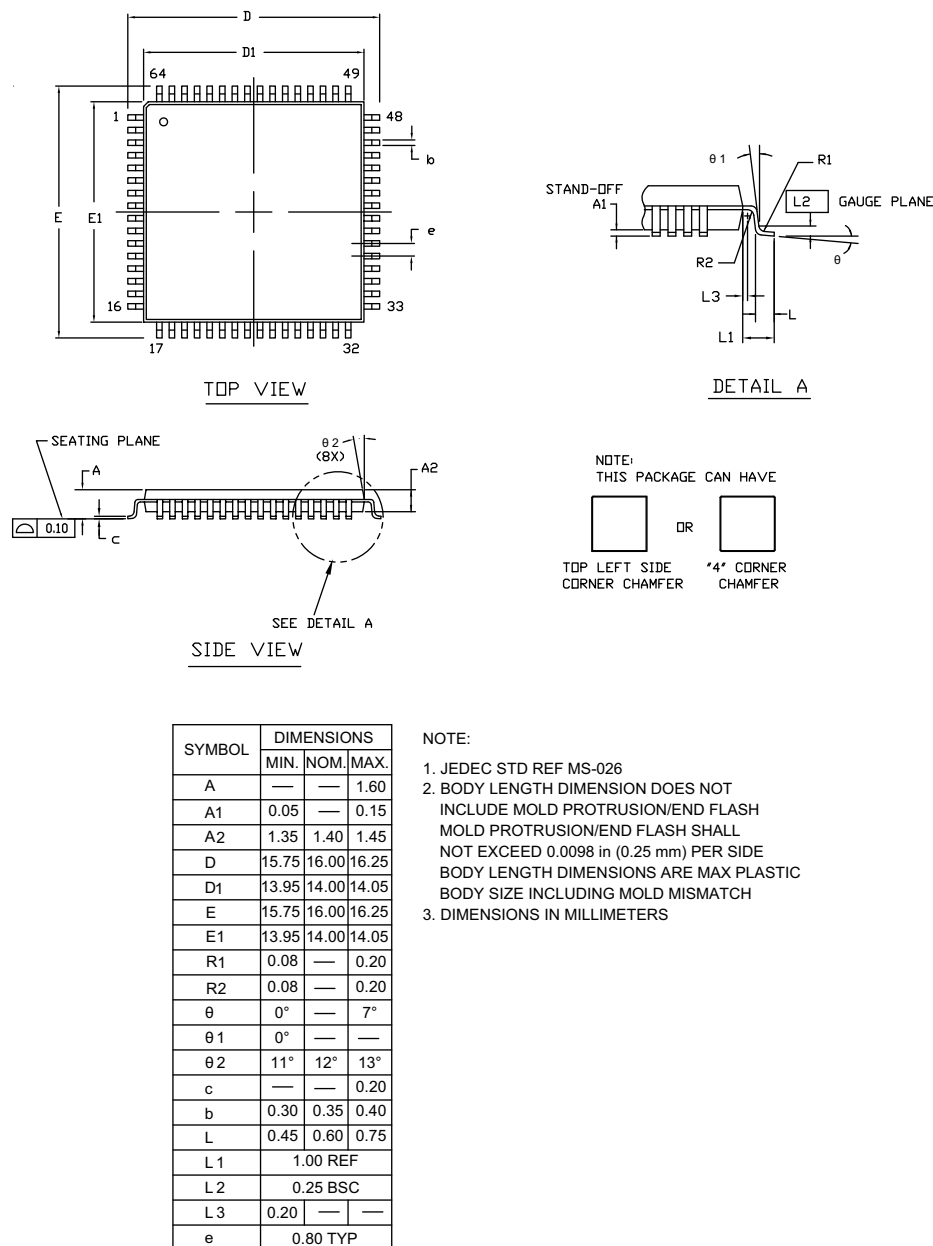
Figure 7 64-pin TQFP package (0.8-mm pitch) outline
