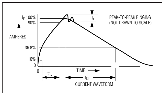
Figure 3b. Human Body Current Waveform
