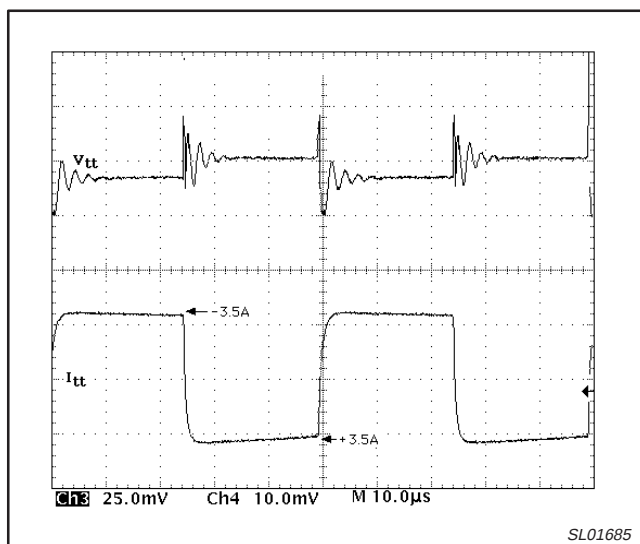
Figure 6. V_{ref} -to- V_{TT} transient response (output filter 50 \mu\text{F} ceramic)
