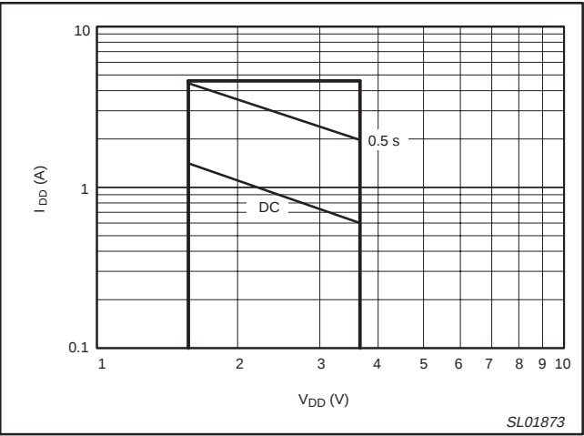
Figure 15. Safe operating area of the NE57814.
