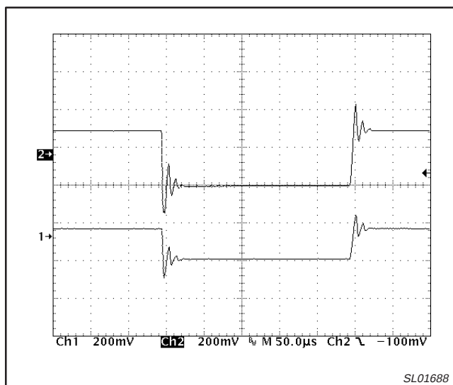
Figure 4. V_{DD} -to- V_{TT} response (output filter 50 \mu\text{F} ceramic)
