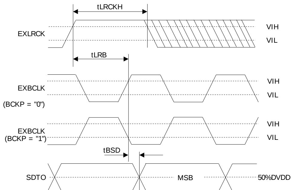
Figure 9. Audio Interface Timing (PLL Slave mode &amp; DSP mode; MSBS = 0)
