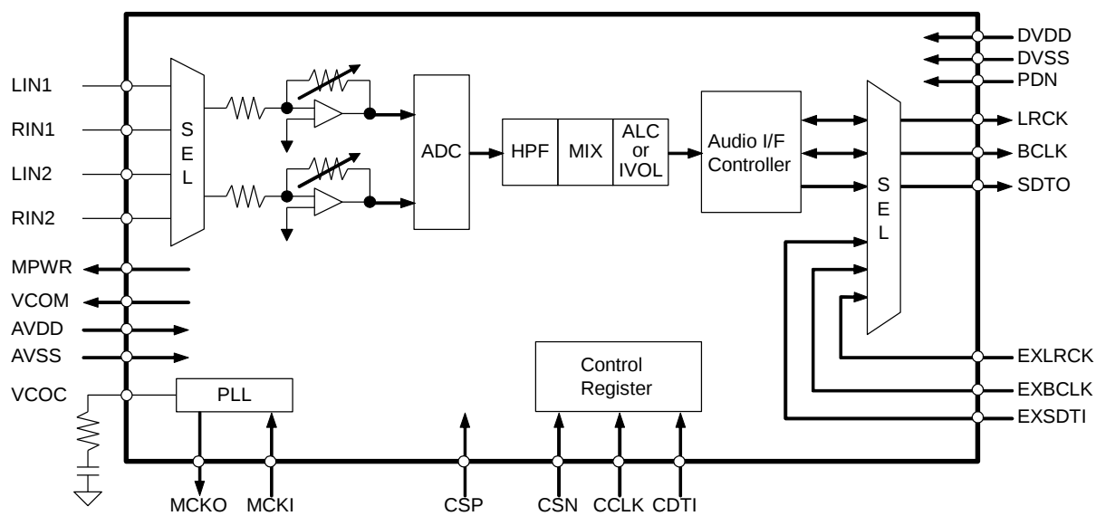
Figure 1. Block Diagram
