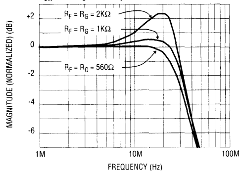
Frequency Response for Various R_F and R_G V_{CM} = 1.5V , R_L = 150\Omega , A_V = +2
