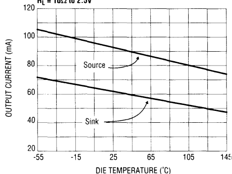
Output Current vs. Die Temperature
