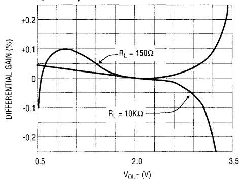
Differential Gain for R_L Tied to 2.5V R_F = 1K\Omega , A_V = +2
