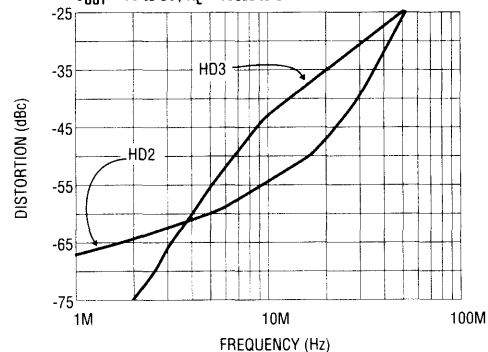
2nd and 3rd Harmonic Distortion vs. Frequency V_{OUT} = 1V to 3V , R_L = 100\Omega to 0V
