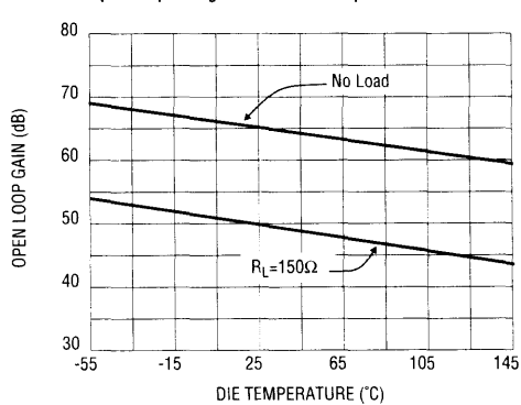
Open Loop Voltage Gain vs. Die Temperature
