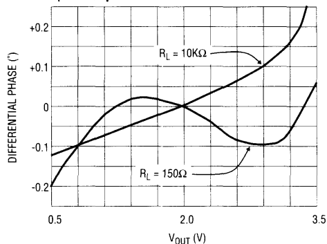
Differential Phase for R_L Tied to 2.5V R_F = 1K\Omega , A_V = +2
