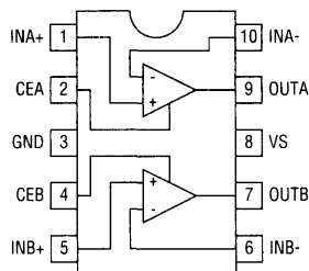
EL5246C (10-Pin MSOP)
