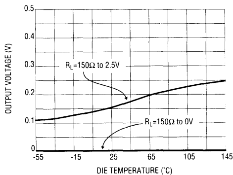
Negative Output Voltage Swing vs. Die Temperature
