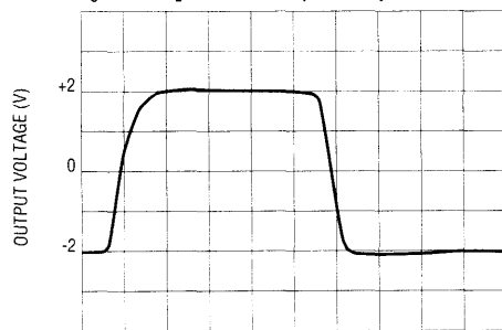
Large Signal Pulse Response (Split Supplies) V_S = \pm 2.5V , R_L = 150\Omega to 0V , R_F = 1K\Omega , A_V = +2
