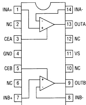
EL5246C (14-Pin SO & 14-Pin PDIP)
