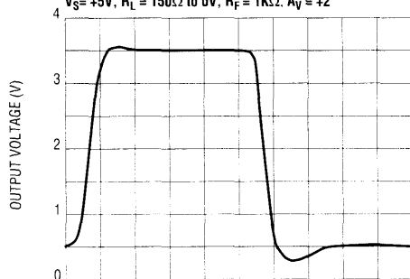
Large Signal Pulse Response (Single Supply) V_S = +5V , R_L = 150\Omega to 0V , R_F = 1K\Omega , A_V = +2
