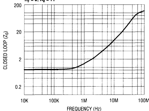
Closed Loop Output Impedance vs. Frequency R_F = 0 , A_V = +1
