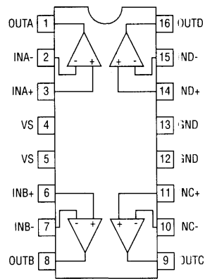
EL5444C (16-Pin QSOP)
