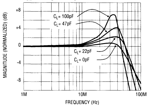
Frequency Response for Various C_L V_{CM} = 1.5V , R_L = 150\Omega , A_V = +1
