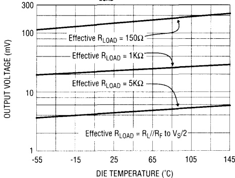
Output Voltage from Either Rail vs. Die Temperature for Various Effective R_{LOAD}
