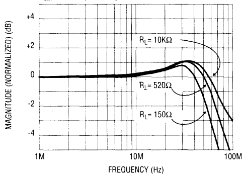
Frequency Response for Various R_L V_{CM} = 1.5V , R_F = 0\Omega , A_V = +1
