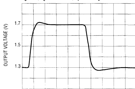
Small Signal Pulse Response (Single Supply) V_S = +5V , R_L = 150\Omega to 0V , R_F = 1K\Omega , A_V = +2
