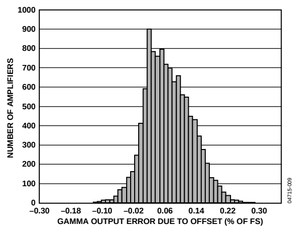
Figure 8. Gamma Output Voltage Error
