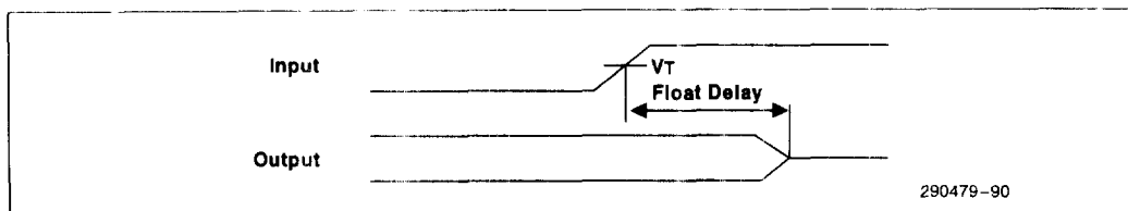
Figure 80. Float Delay
