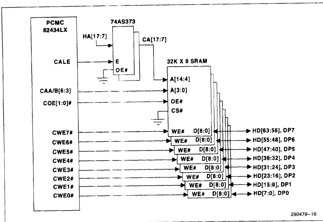
Figure 14. 82434LX Connections to 256-KByte Cache with Standard SRAM
