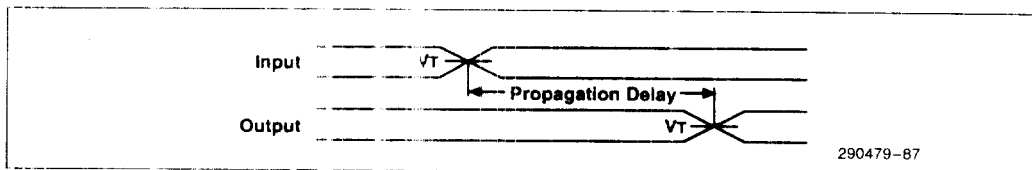
Figure 77. Propagation Delay
