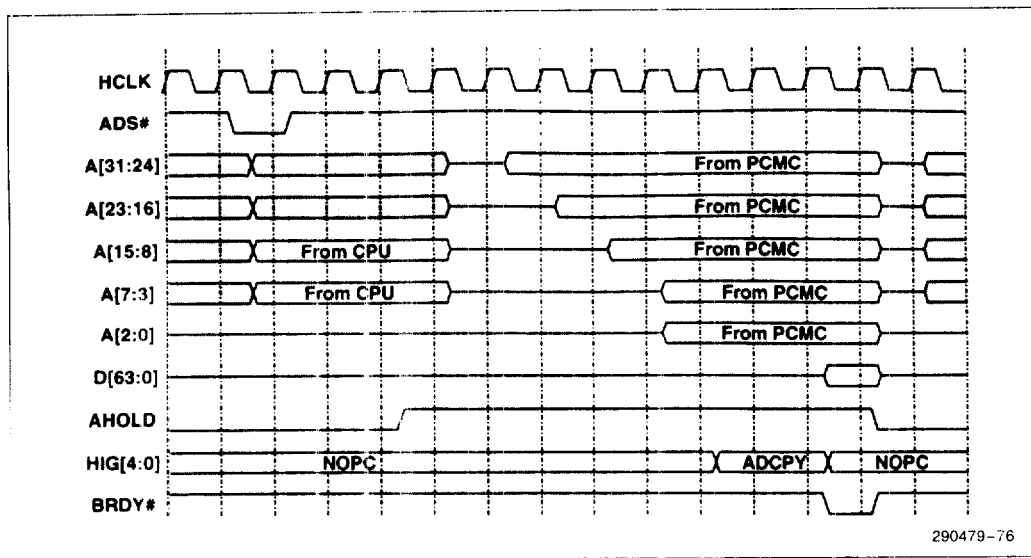
Figure 66. CPU Read from PCMC Configuration Register
