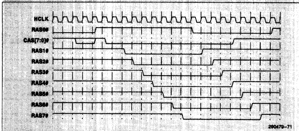
Figure 62. CAS#-Before-RAS# Refresh—Single
