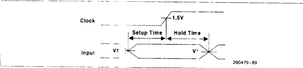
Figure 79. Setup and Hold Times
