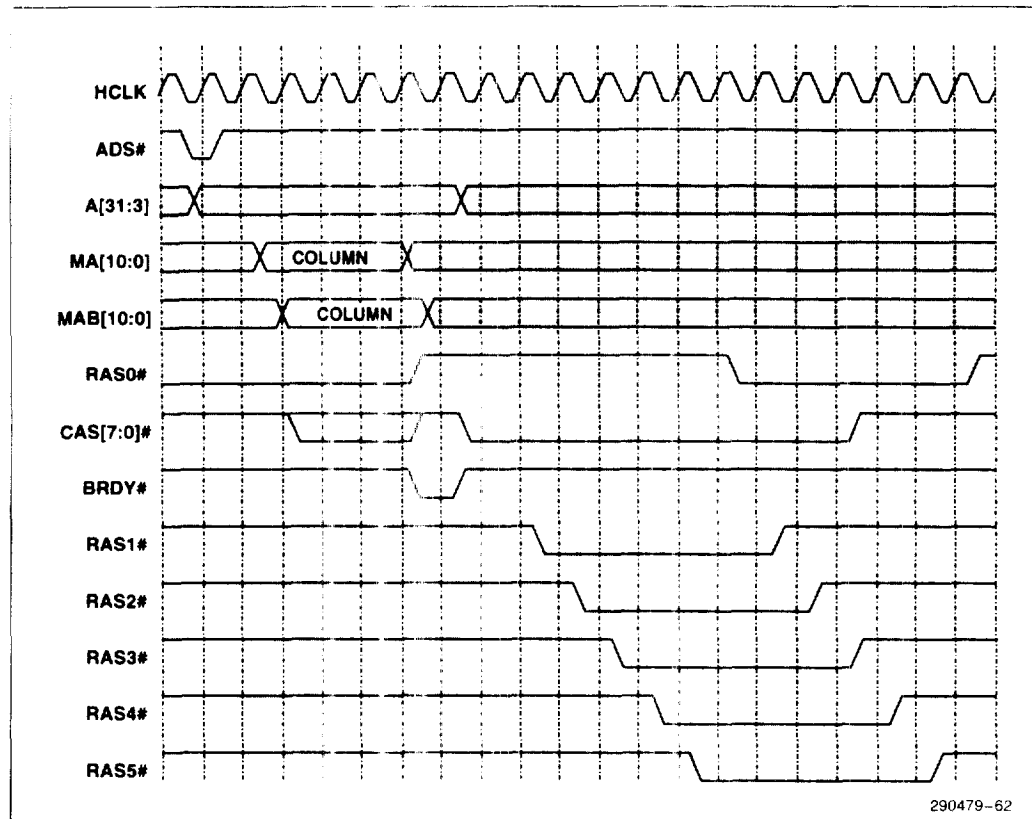
Figure 53. CAS#-before-RAS# Refresh-Single
