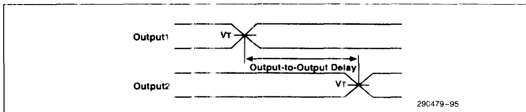
Figure 85. Output-to-Output Delay
