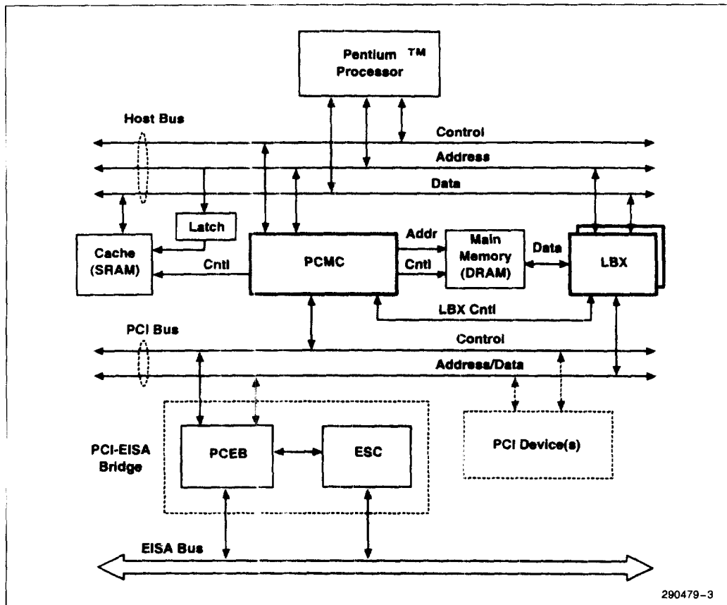
Figure 2. Block Diagram of the 82430LX/82430NX PCIsset EISA System
