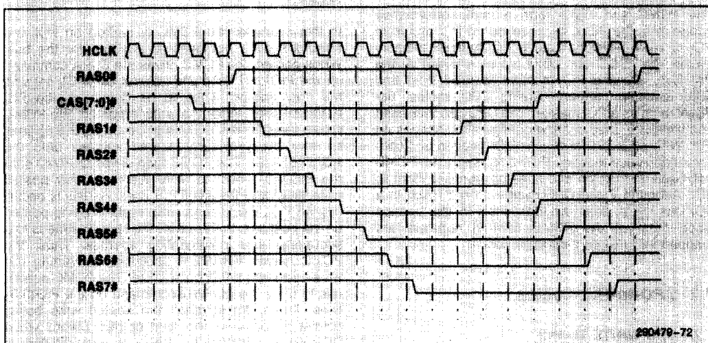
Figure 63. Hidden Refresh—Single
