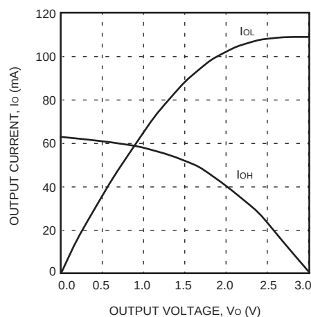
Figure 103. Fast ( T_J = 125^\circ\text{C} , V_{DD} = 3.0\text{ V} )
