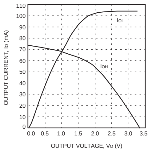
Figure 98. Sinklim ( T_J = 25^\circ\text{C} , V_{DD} = 3.3\text{ V} )
