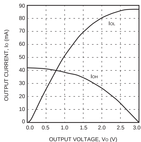
Figure 101. Sinklim ( T_J = 125^\circ\text{C} , V_{DD} = 3.0\text{ V} )
