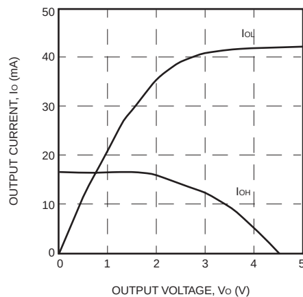
Figure 95. Sinklim ( T_J = 125^\circ\text{C} , V_{DD} = 4.5\text{ V} )
