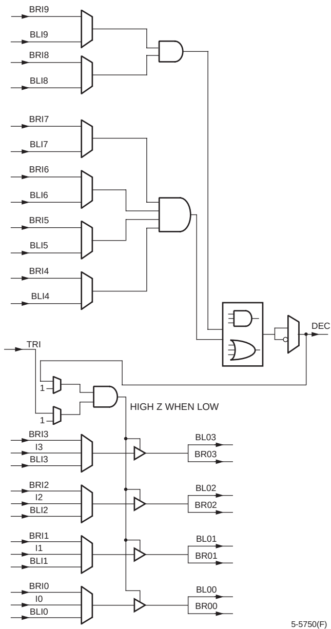
Figure 15. Buffer-Decoder-Decoder Mode
