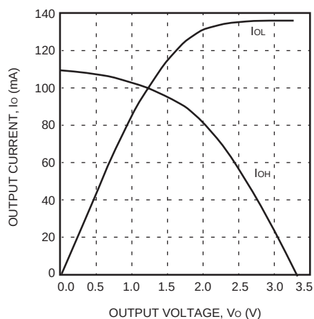
Figure 100. Fast ( T_J = 25^\circ\text{C} , V_{DD} = 3.3\text{ V} ) Lattice Semiconductor
