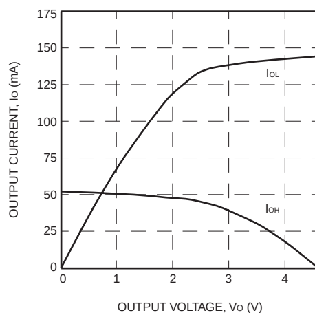
Figure 97. Fast ( T_J = 125^\circ\text{C} , V_{DD} = 4.5\text{ V} )
