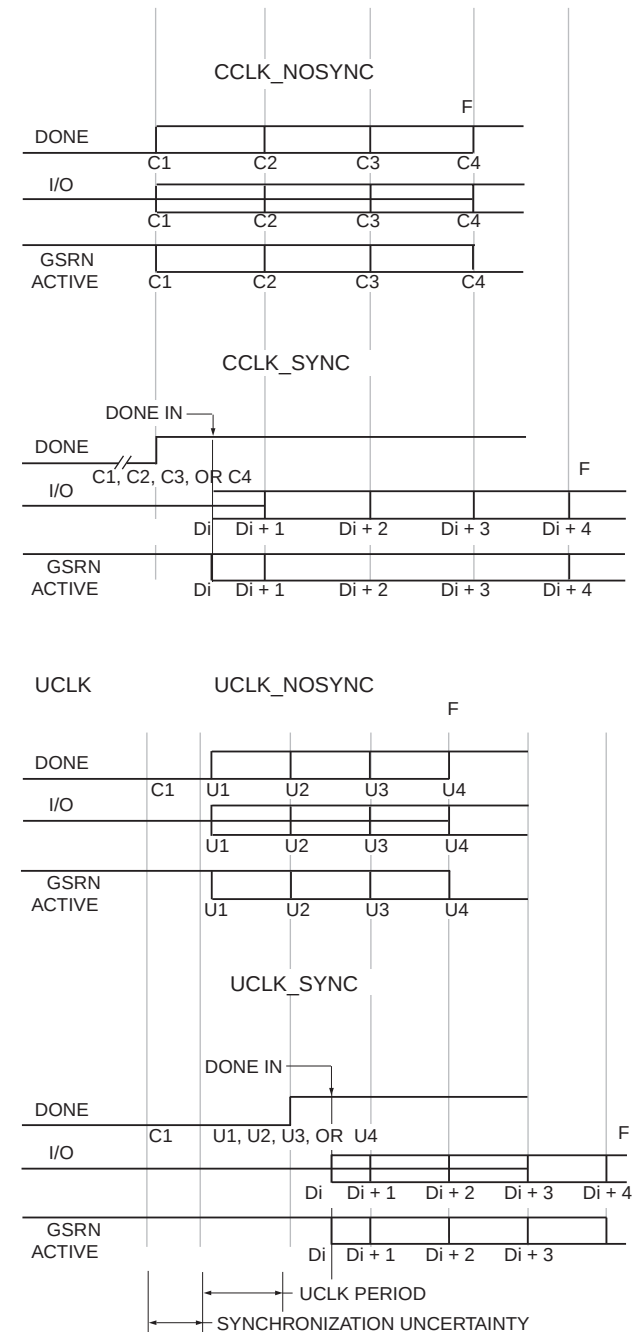
Figure 51. Start-Up Waveforms
