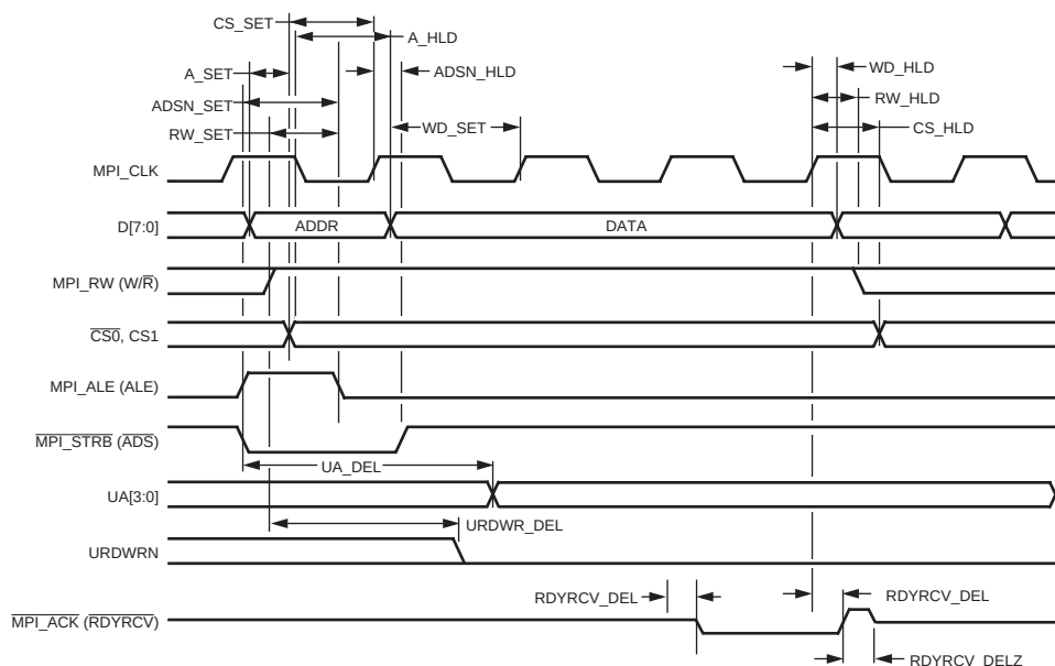
Figure 74. MPI i960 Internal Write Timing
