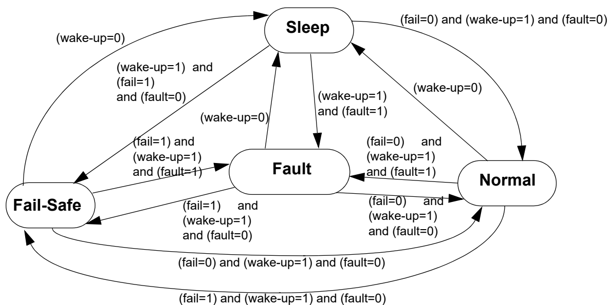
Figure 12. Operating modes
