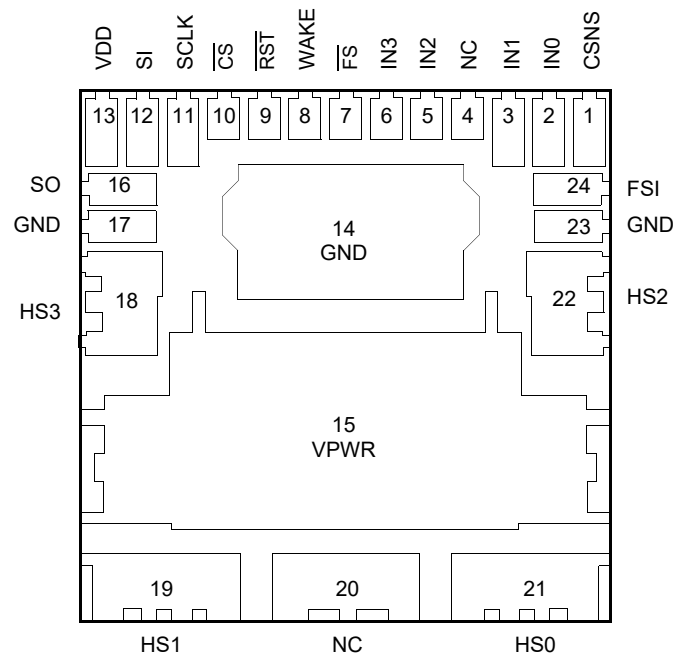
Figure 23. Pin connections
