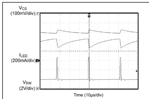
FIGURE 2-25: Steady-State Operation at V_{IN} = 4.5V .
