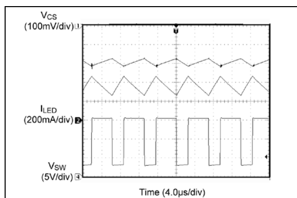
FIGURE 2-26: Steady-State Operation at V_{IN} = 12V .
