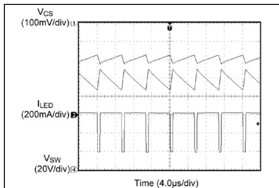
FIGURE 2-28: Steady-State Operation at V_{IN} = 42V .
