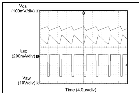
FIGURE 2-27: Steady-State Operation at V_{IN} = 24V .
