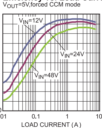
Efficiency vs. Load Current
