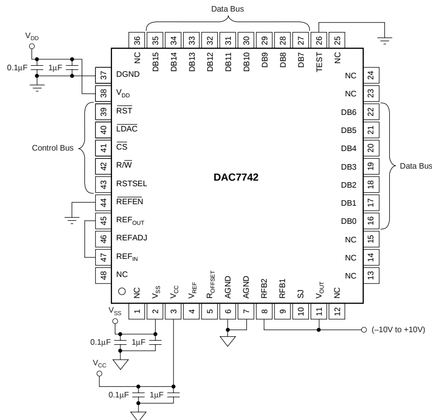
FIGURE 4. Basic Operation: V_{OUT} = -10V to +10V .
