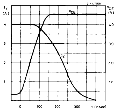
Figure 6. Turn-off Phase.
