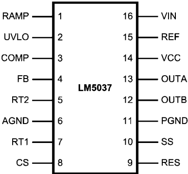
Top View 16-Lead TSSOP Package
