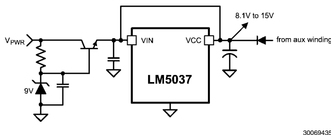
FIGURE 11. Start-up Regulator for V_{PWR} > 100V
