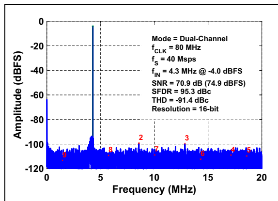
FIGURE 3-5: FFT for 4.3 MHz Input Signal: f_S = 40 Msps, Dual-Ch., A_{IN} = -4 dBFS.
