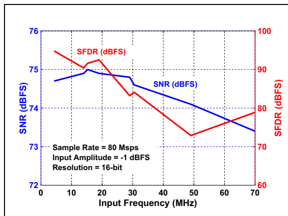
FIGURE 3-31: SNR/SFDR vs. Input Frequency: f_S = 80 Mpsps.
