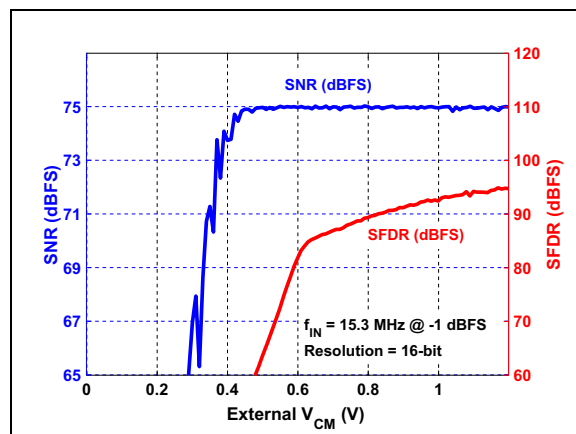
FIGURE 3-34: SNR/SFDR vs. V_{CM} Voltage (Externally Applied): f_S = 80 Mpsps, f_{IN} = 15.3 MHz.
