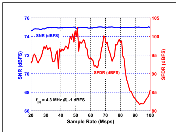
FIGURE 3-30: SNR/SFDR vs. Sample Rate (Mpsps): f_{IN} = 4.3 MHz.
