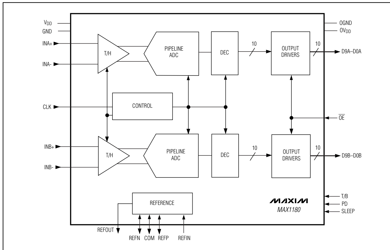
Functional Diagram
