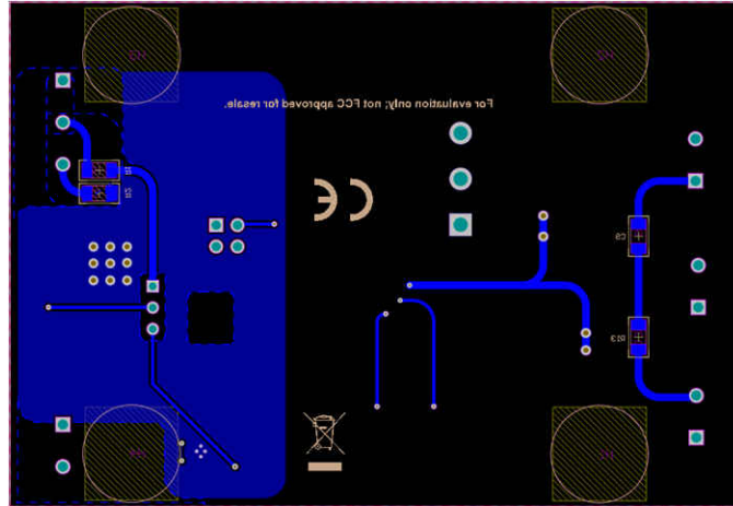
Figure 11-3. Bottom Layer
