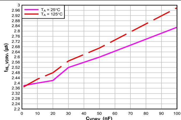
Figure 6-5. t HL_VDRV , Three-Wire Mode, TPSI3050-Q1
