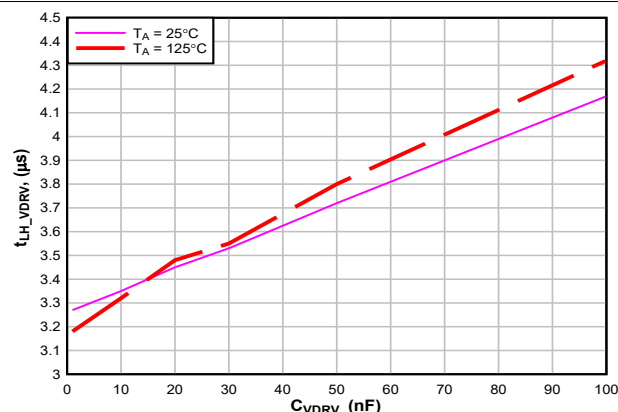
Figure 6-4. t LH_VDRV , Three-Wire Mode, TPSI3050-Q1
