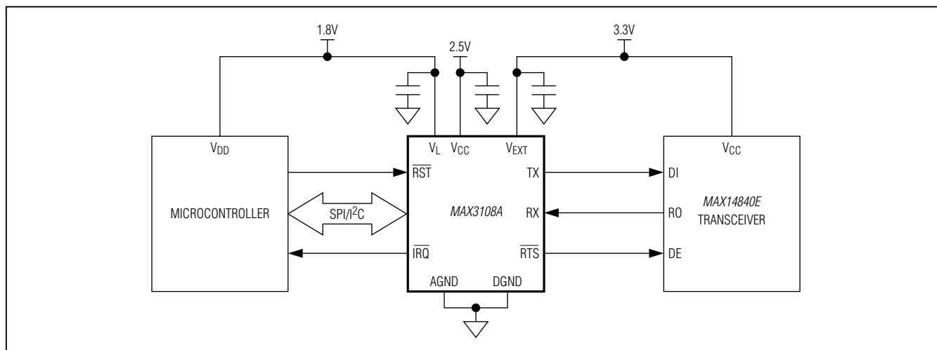
Figure 24. Logic-Level Translation
