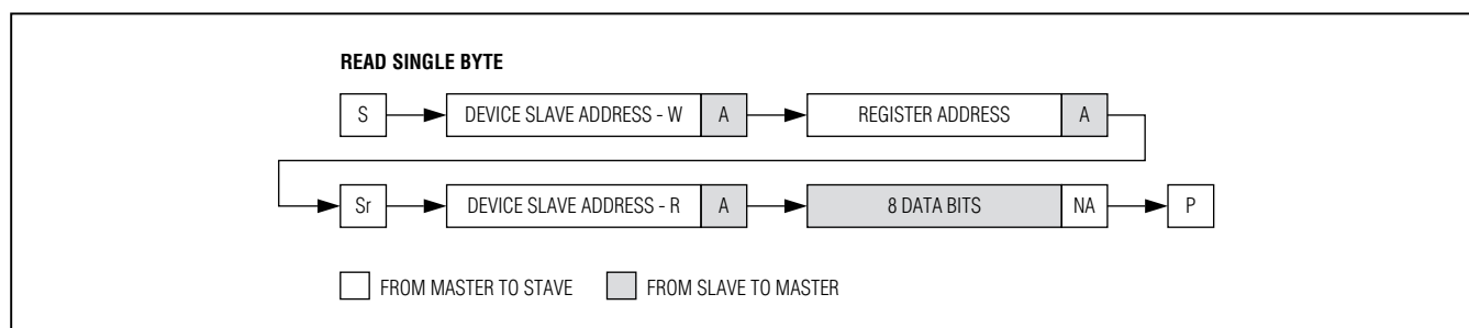
Figure 20. Read Byte Sequence
