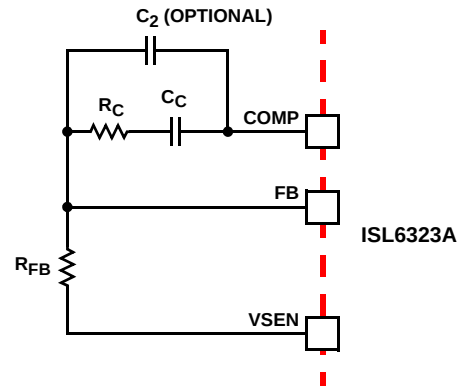
FIGURE 22. COMPENSATION CONFIGURATION FOR LOAD-LINE REGULATED ISL6323A CIRCUIT
