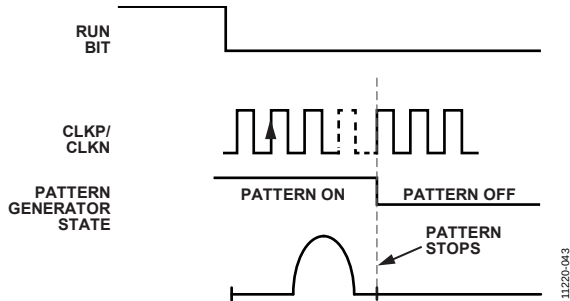
Figure 43. RUN Bit Driven Pattern Stop
