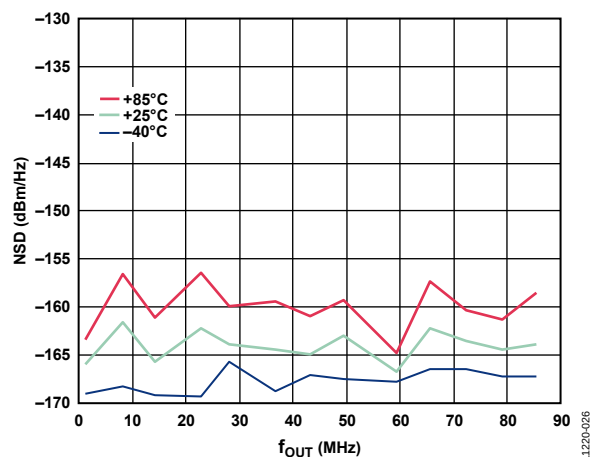
Figure 26. NSD vs. f_{OUT} at Three Temperatures
