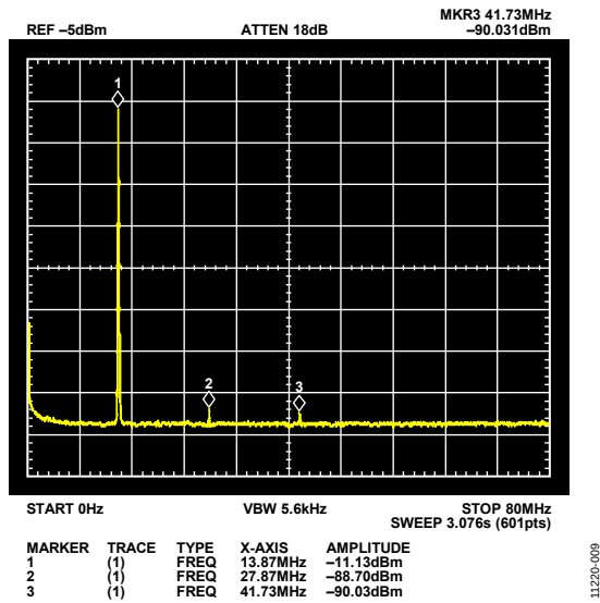
Figure 9. Output Spectrum, f_{OUT} = 13.87 MHz
