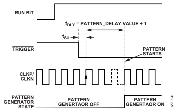
Figure 41. TRIGGER Pin Initiated Pattern Start with Pattern Delay
