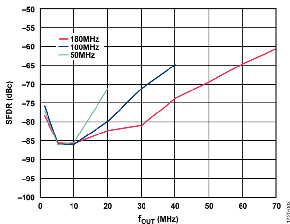
Figure 8. SFDR at Three f_{DAC} Values vs. f_{OUT}
