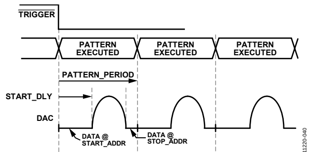
Figure 40. Periodic Pulse Trains Output on All DACs
