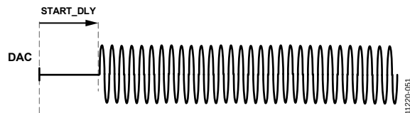
Figure 51. Waveform with Start Delays
