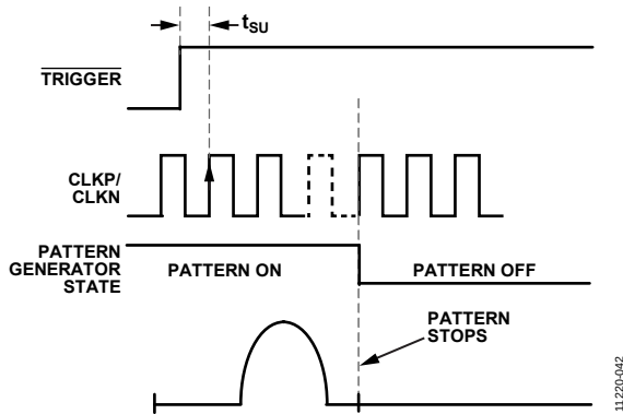
Figure 42. Trigger Rising Edge Initiated Pattern Stop
