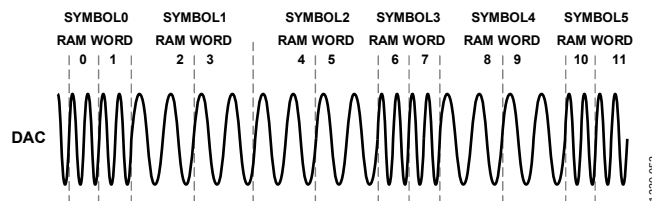
Figure 53. FSK Modulated Signal
