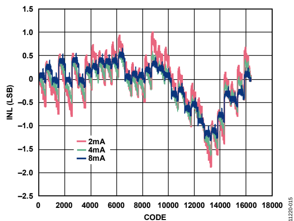
Figure 15. INL, Three I_{OUTS} Values
