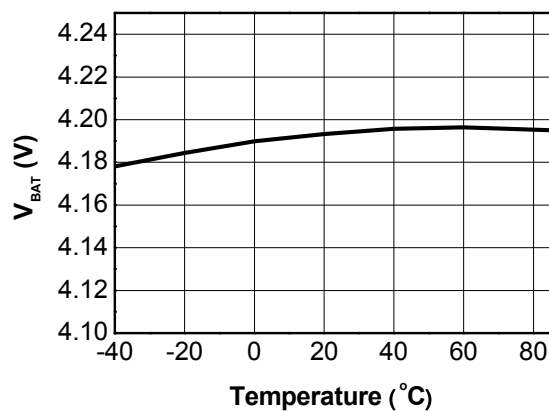
Figure 26. V_{BAT} vs T_A V_{USB}=5.0 V, I_{BAT}=0 mA
