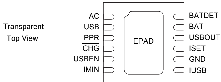
Figure 3. 34676 Pin Connections
