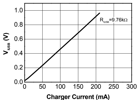
Figure 20. V_{IUSB} vs USB Charger Charge Current V_{USB}=5.0 V, T_A=25^\circ\text{C}
