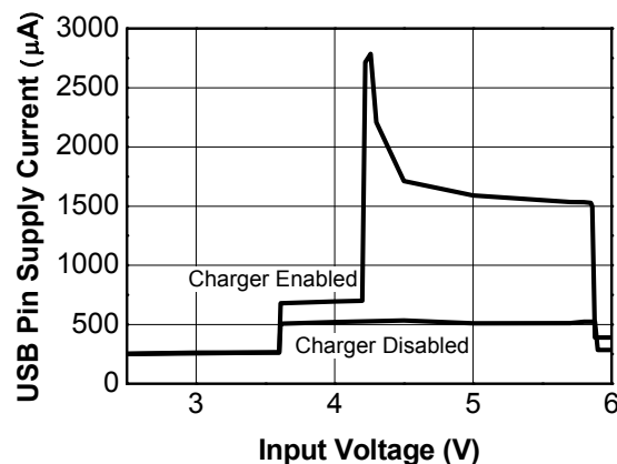
Figure 18. USB Pin Supply Current vs V_{USB} I_{BAT}=0 mA, T_A=25^\circ\text{C}
