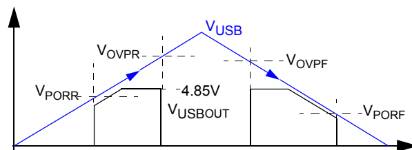
Figure 39. Voltage Regulated Output vs. Input Voltage
