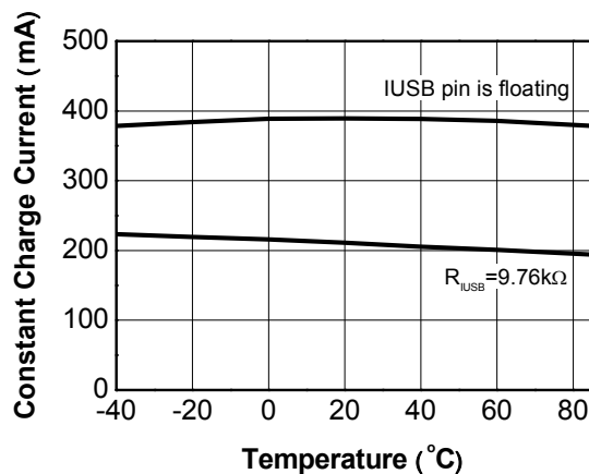
Figure 30. USB Charger CC Current vs T_A V_{USB}=5.0 V, V_{BAT}=3.7 V
