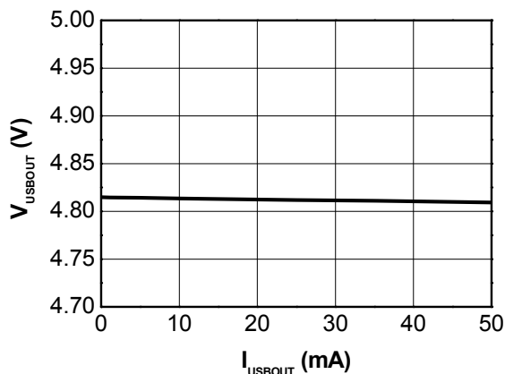
Figure 24. V_{USBOUT} vs I_{USBOUT} V_{USB}=5.0 V, T_A=25^\circ\text{C}
