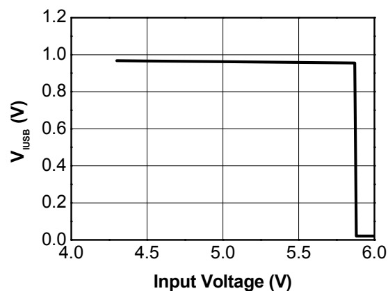
Figure 19. V_{IUSB} vs V_{USB} V_{BAT}=3.7 V, R_{IUSB}=9.76 k \Omega , T_A=25^\circ\text{C}
