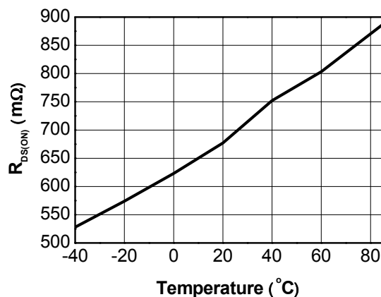
Figure 29. USB Charger R_{DS(ON)} vs T_A V_{BAT}=4.0 V, I_{USB}=400 mA, I_{BAT}=300 mA
