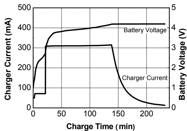
Figure 17. USB Charger Complete Charge Cycle V_{USB}=5.0 V, R_{IUSB}=6.52 k \Omega , 740 mA Battery, T_A=25^\circ\text{C}
