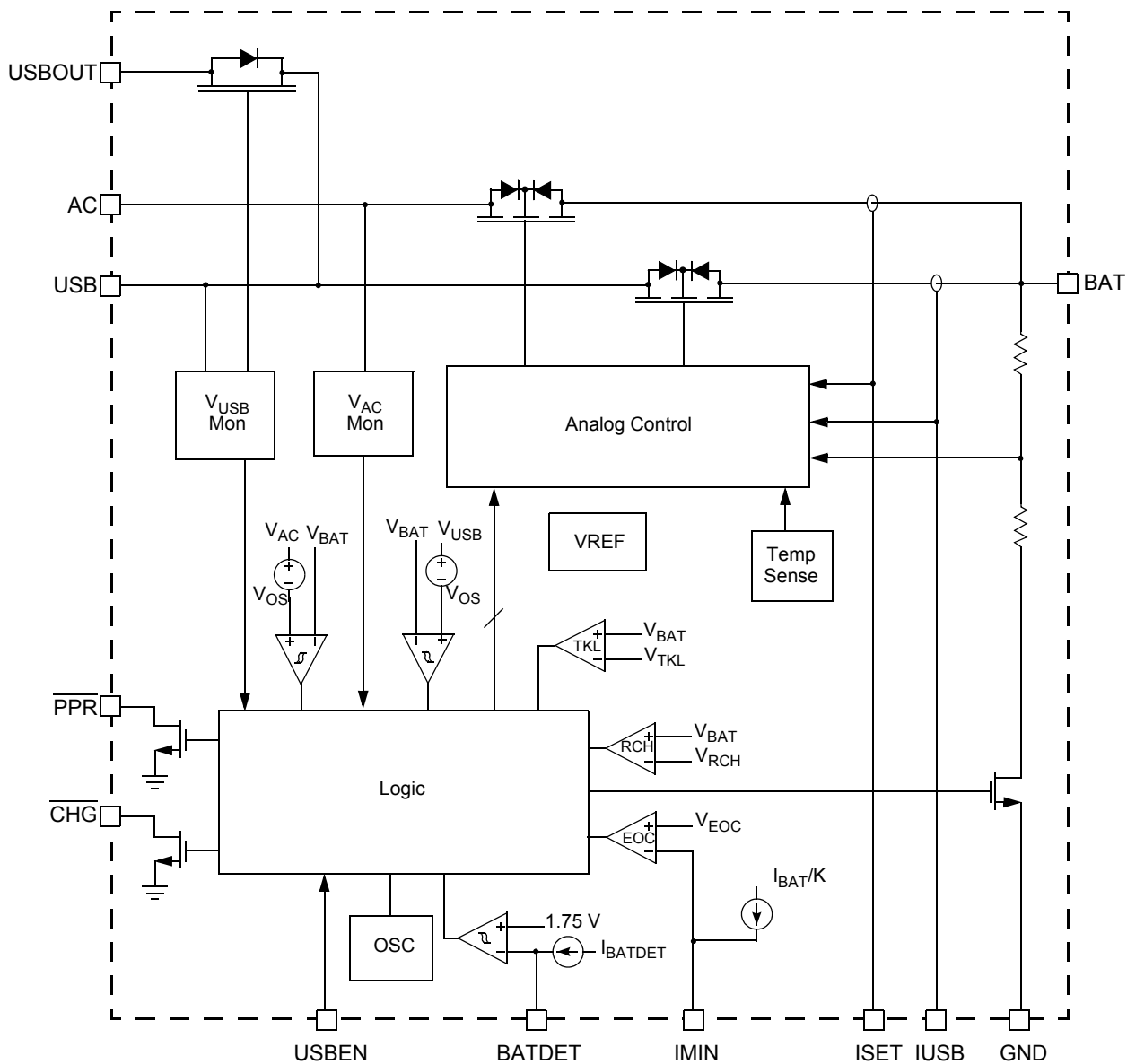
Figure 2. 34676 Simplified Internal Block Diagram
