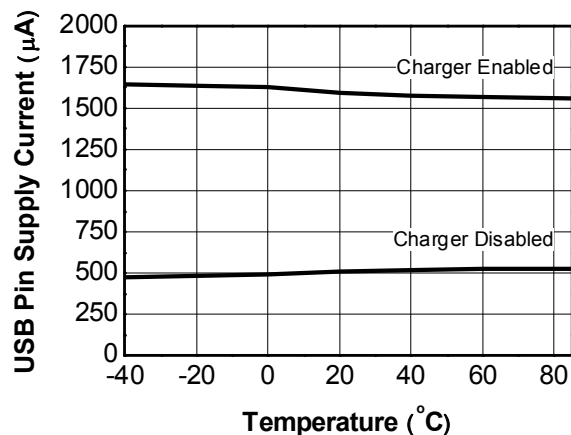
Figure 27. USB Pin Supply Current vs T_A V_{USB}=5.0 V, I_{BAT}=0 mA
