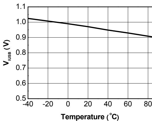
Figure 28. V_{IUSB} vs T_A V_{USB}=5.0 V, R_{IUSB}=9.76 kΩ, V_{BAT}=3.7 V
