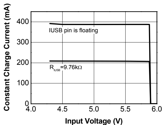
Figure 21. USB Charger CC Current vs V_{IUSB} V_{BAT}=3.7 V, T_A=25^\circ\text{C}
