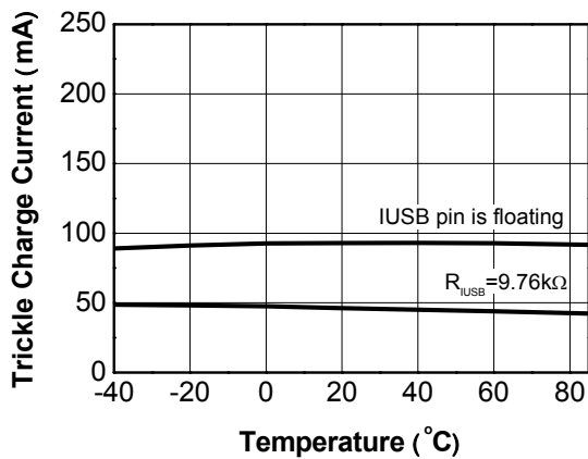
Figure 31. USB Charger Trickle Current vs T_A V_{USB}=5.0 V, V_{BAT}=2.0 V
