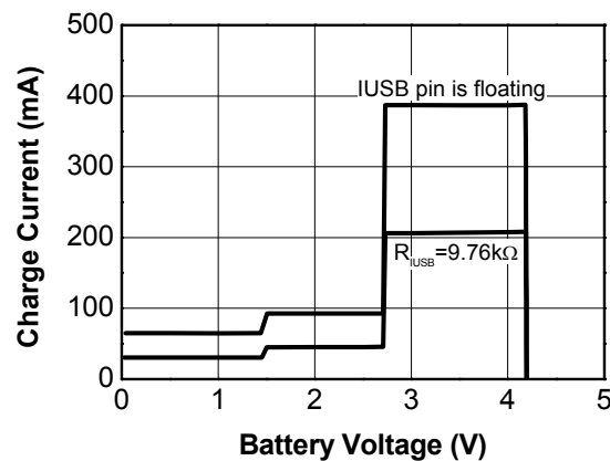
Figure 22. USB Charger Charge Current vs V_{BAT} V_{USB}=5.0 V, T_A=25^\circ\text{C}
