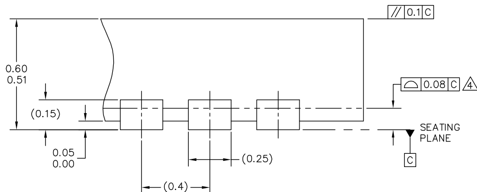
DETAIL G
