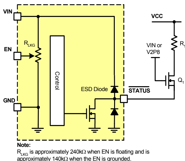
FIGURE 23. PULL-UP CIRCUIT TO AVOID BATTERY LEAKAGE CURRENT IN THE ESD DIODES
