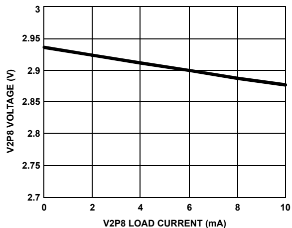
FIGURE 8. V2P8 OUTPUT vs ITS LOAD CURRENT
