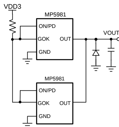
Figure 13: GOK and ON/PD Connection Parallel Devices
