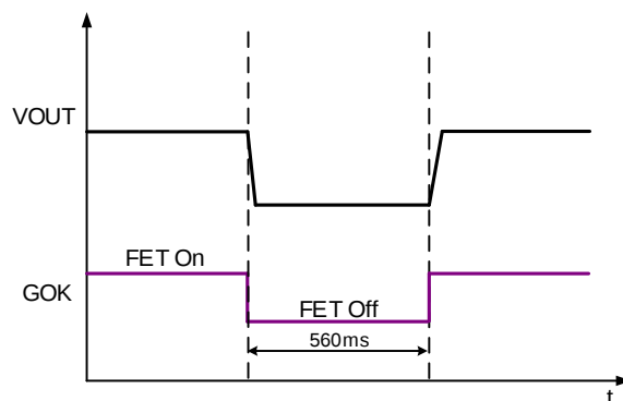
Figure 12: Auto-Retry Operation
