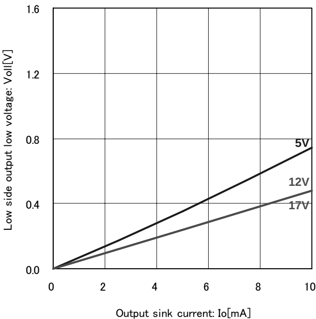
Fig.10 Low side output low voltage ( T_a=25^{\circ}\text{C} )
