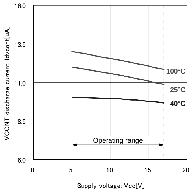
Fig.30 VCONT discharge current
