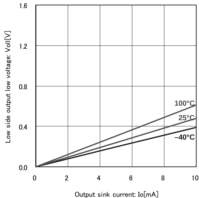
Fig.9 Low side output low voltage ( V_{cc}=12\text{V} )
