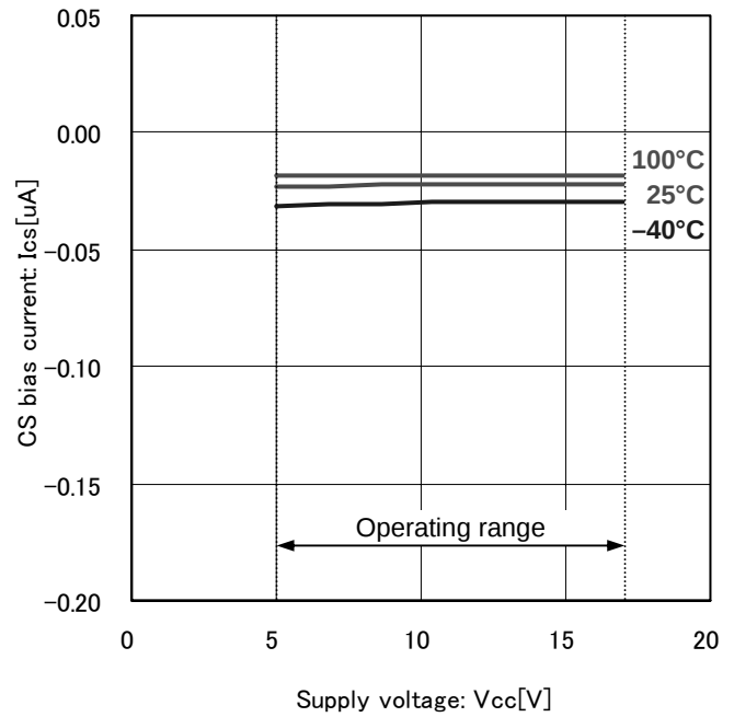
Fig.24 CS bias current
