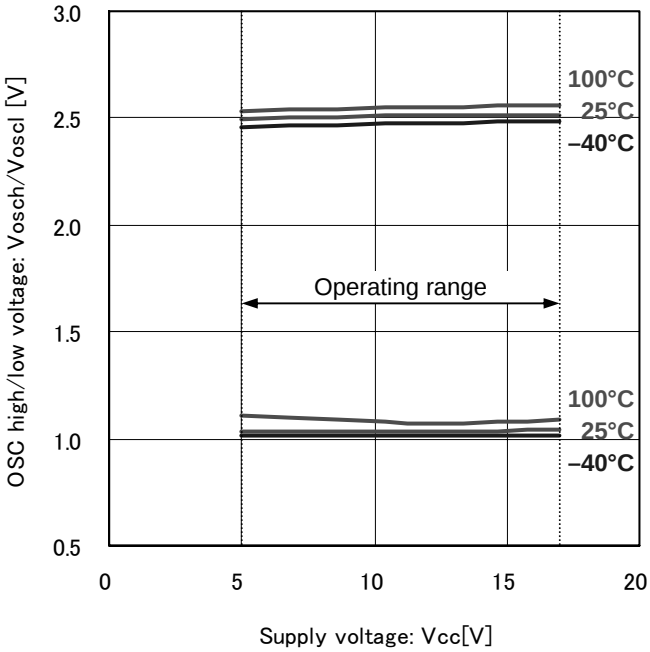
Fig.16 OSC high/low voltage
