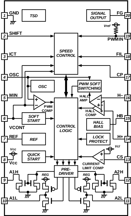
Fig.2 Block diagram
