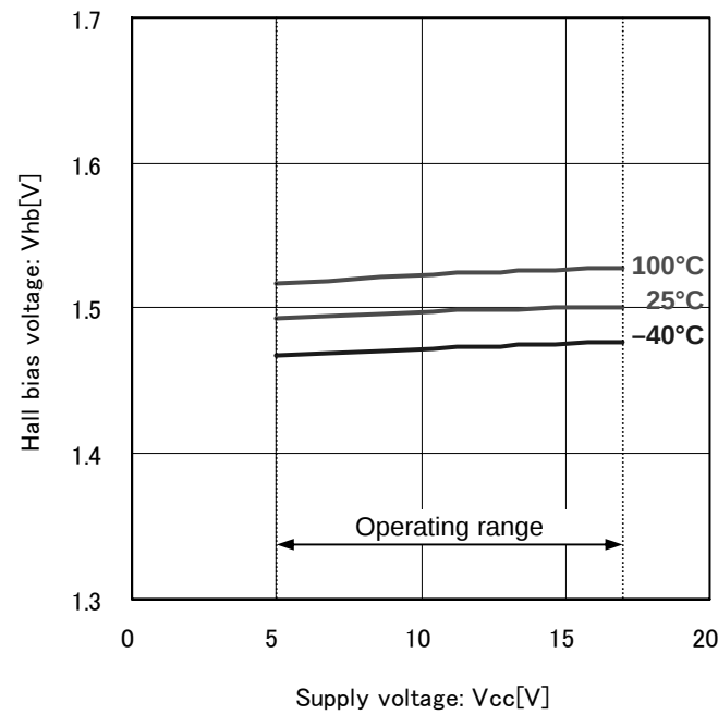
Fig.20 Hall bias voltage
