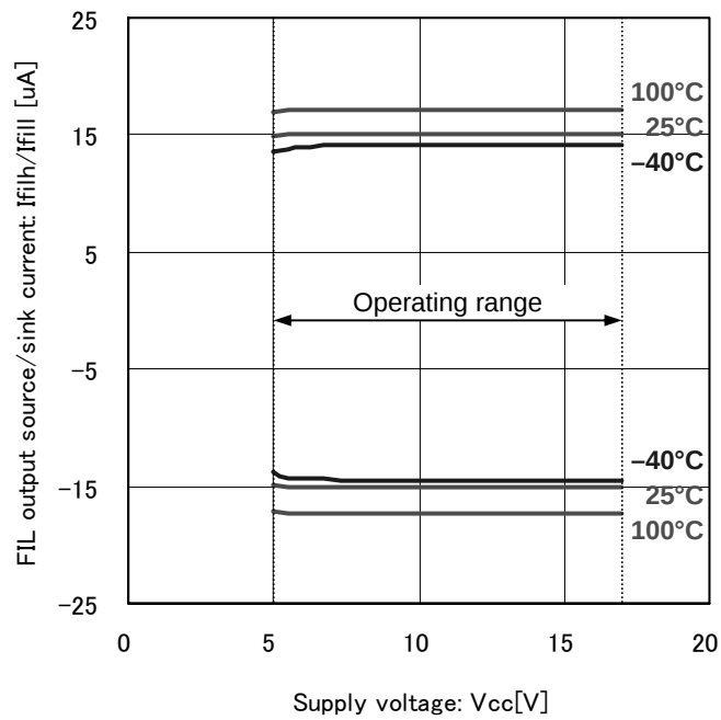
Fig.28 FIL output source/sink current
