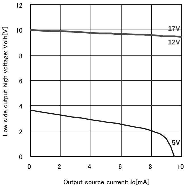
Fig.8 Low side output high voltage ( T_a=25^{\circ}\text{C} )
