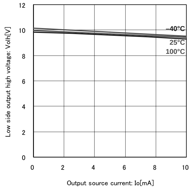
Fig.7 Low side output high voltage ( V_{cc}=12\text{V} )
