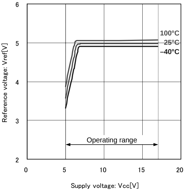
Fig.18 Reference voltage
