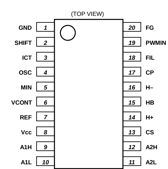
Fig.1 Pin configuration
