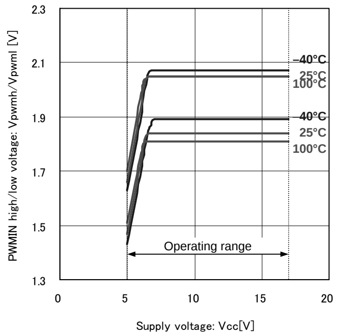
Fig.26 PWMIN input high/low voltage
