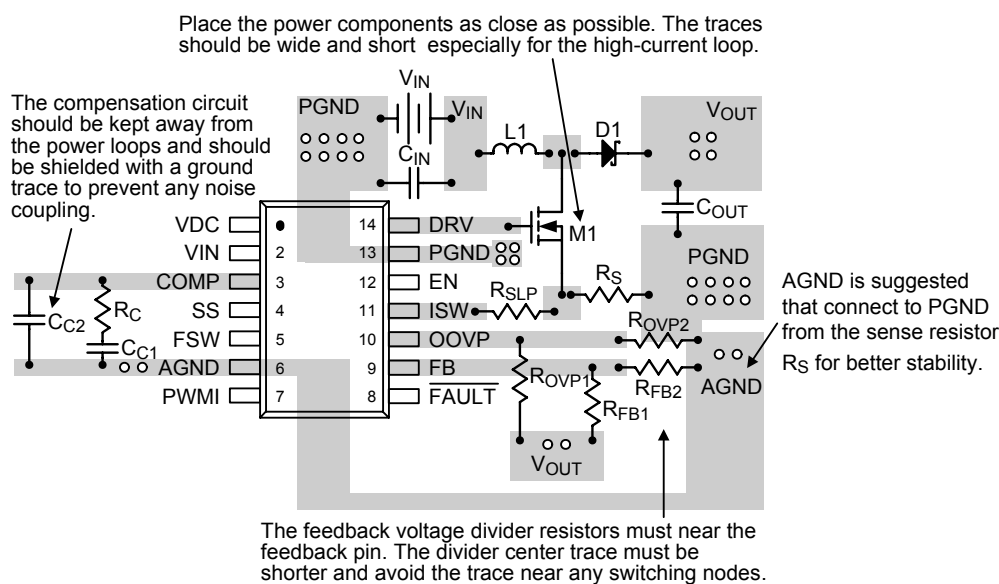
Figure 5. PCB Layout Guide
