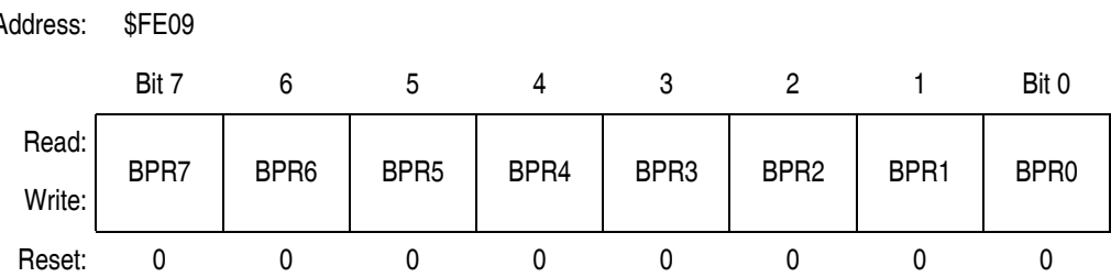
Figure 4-4. FLASH Block Protect Register (FLBPR)
