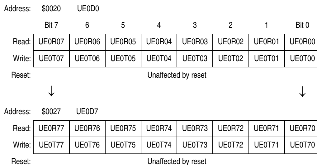
Figure 11-26. USB Endpoint 0 Data Registers (UE0D0–UE0D7)
