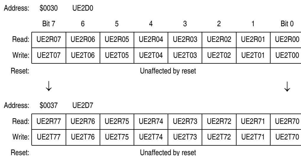
Figure 11-28. USB Endpoint 2 Data Registers (UE2D0–UE2D7)
