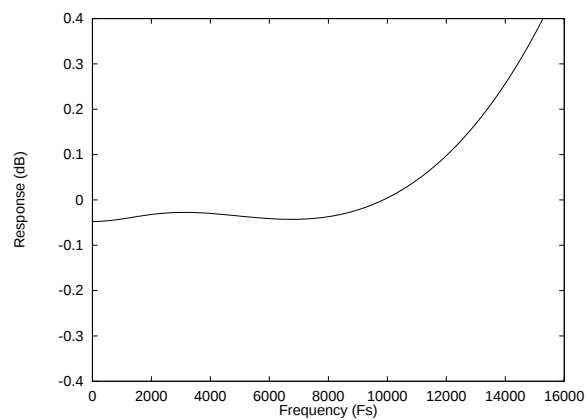
Figure 45 De-emphasis Error (32kHz)
