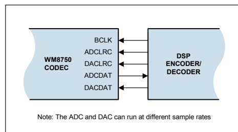
Figure 17 Slave Mode
