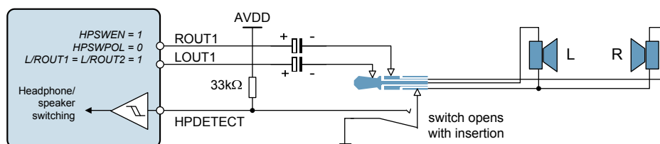
Figure 11 Example Headset Detection Circuit Using Normally-Open Switch
