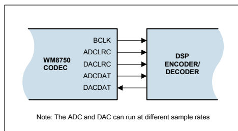
Figure 16 Master Mode
