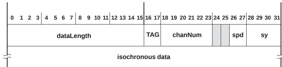
Figure 3–36. Isochronous-Transmit Format
