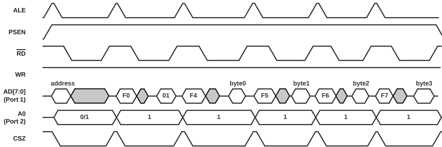
Figure 4-30. Intel 8051 Read Timing (Blind Access Read)
