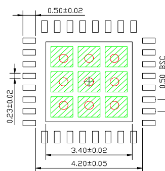
RECOMMENDED LAND PATTERN NOTE: 4, 5
