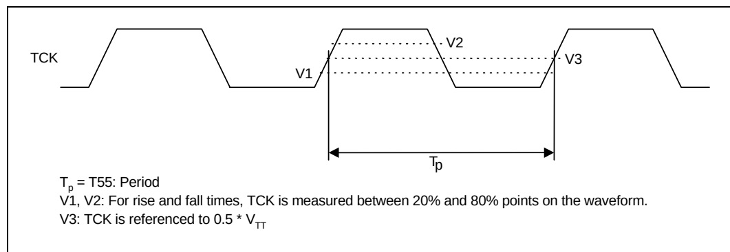
Figure 2-14. TCK Clock Waveform
