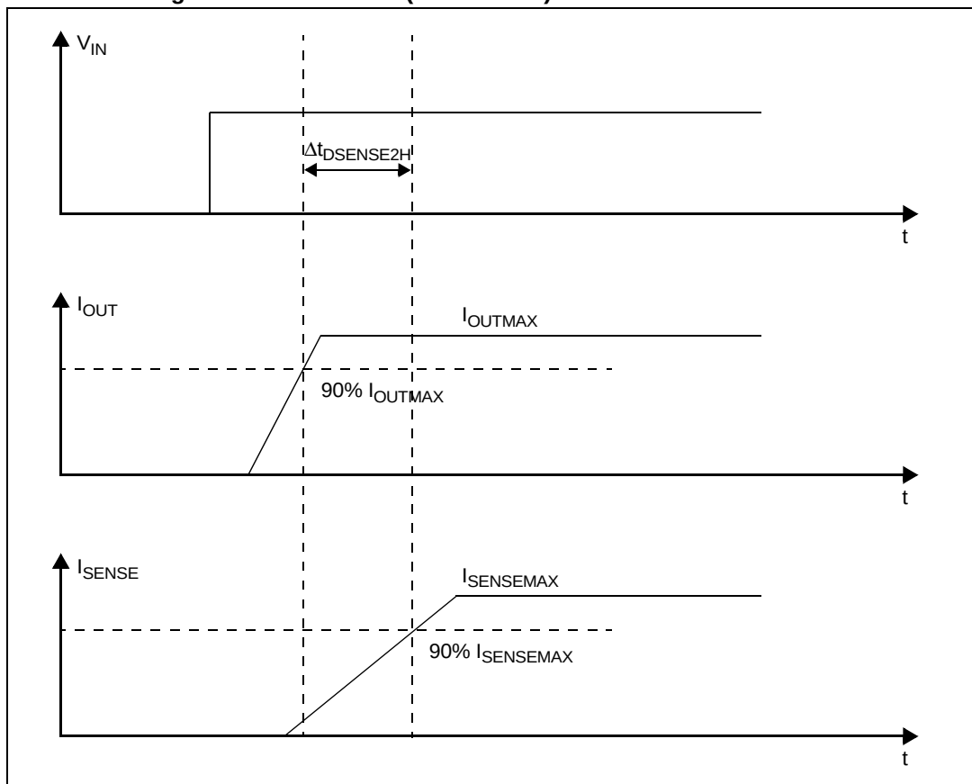
Figure 6. Switching characteristics
