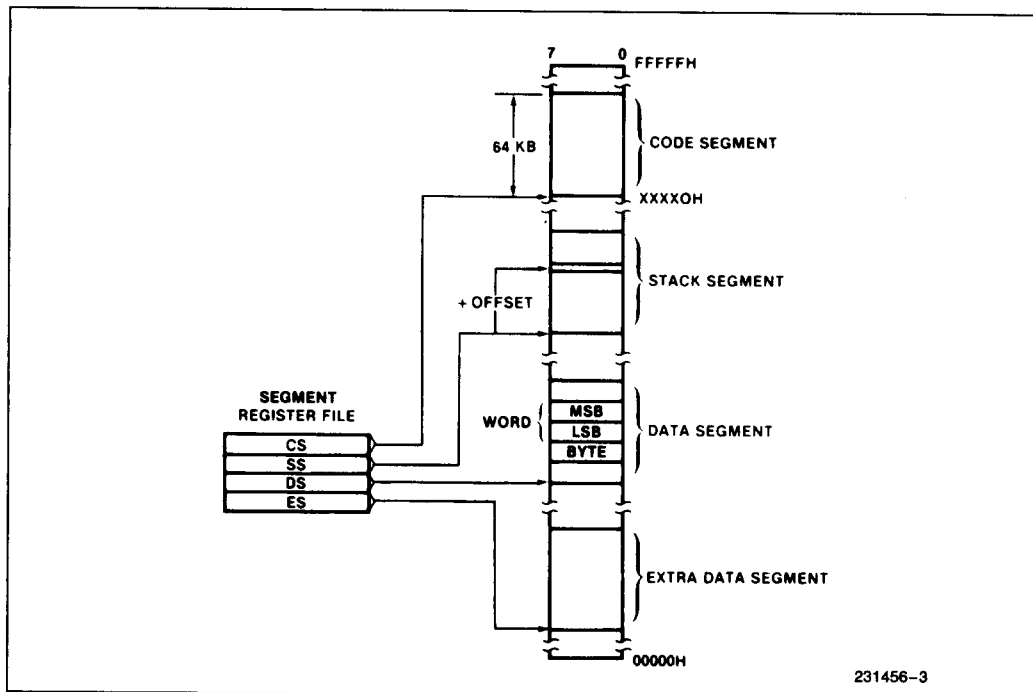
Figure 3. Memory Organization
