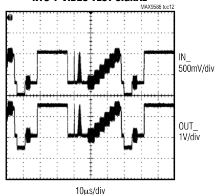
NTC-7 VIDEO TEST SIGNAL
