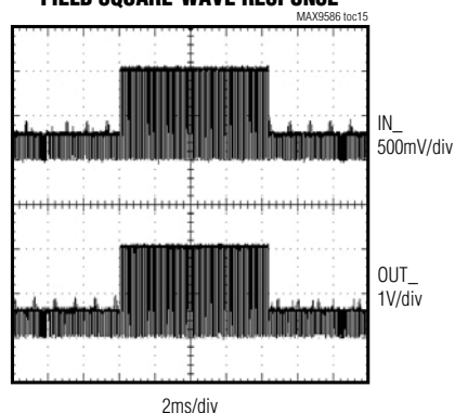
FIELD SQUARE-WAVE RESPONSE
