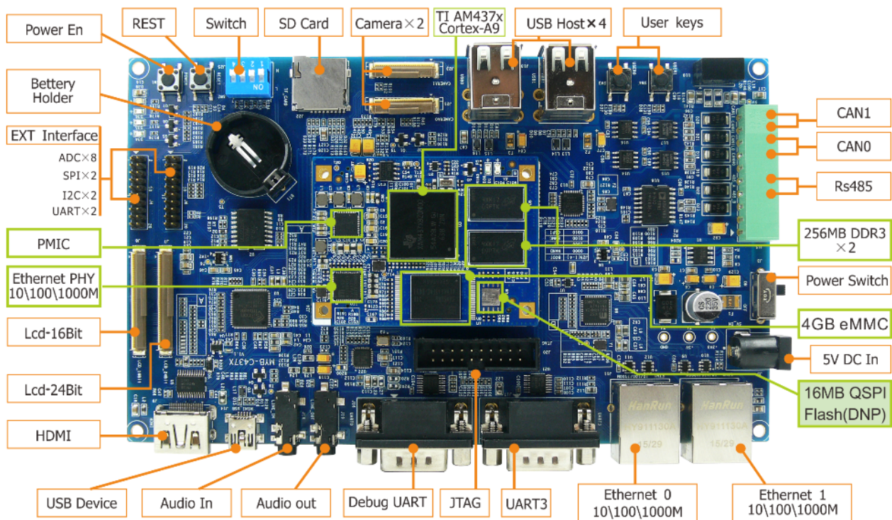
Figure 1-5 MYD-C437X Development Board
