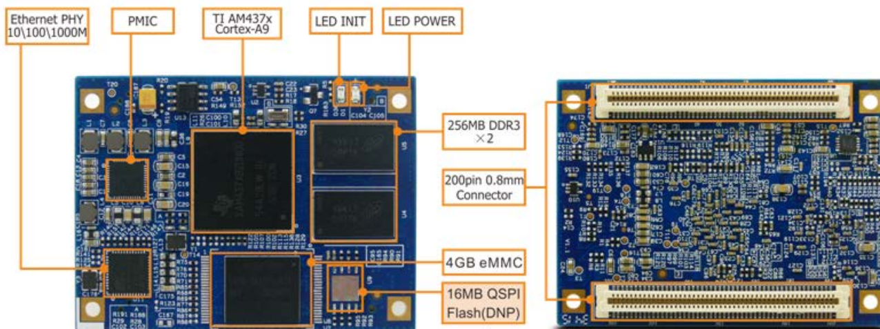
Figure 1-3 MYC-C437X CPU Module
