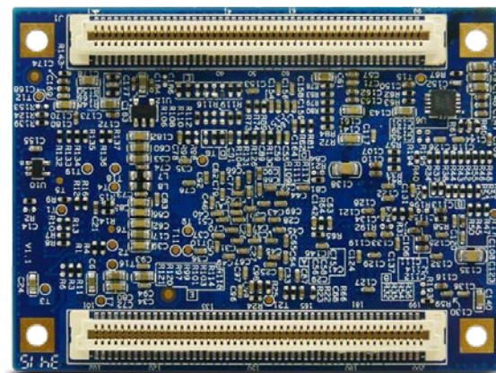
Figure 1-2 MYC-C437X CPU Module Bottom-view
