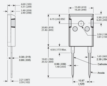
TO-247 2-Lead
