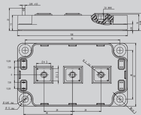
SP6—Three Outputs
