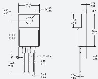
TO-220 [KF]
