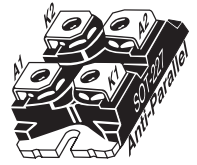
SOT-227 Antiparallel Configuration (Isolated Base)
