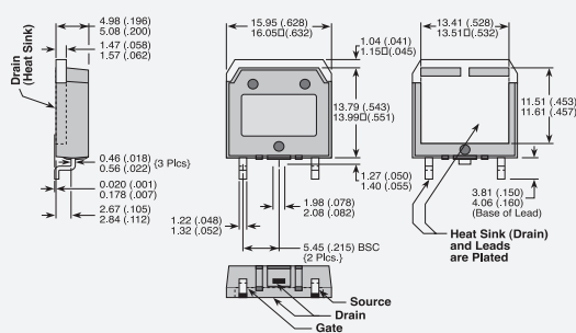
TO-220 [KF]
