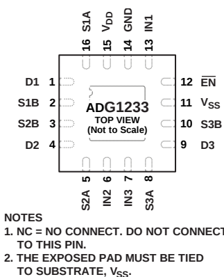
Figure 5. 16-Lead, 4 mm × 4 mm LFCSP Pin Configuration, Exposed Pad Tied to Substrate, V_{SS}
