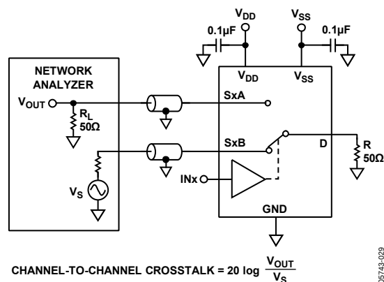
Figure 33. Channel-to-Channel Crosstalk
