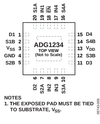
Figure 6. 20-Lead, 4 mm × 4 mm LFCSP Pin Configuration, Exposed Pad Tied to Substrate, V_{SS}
